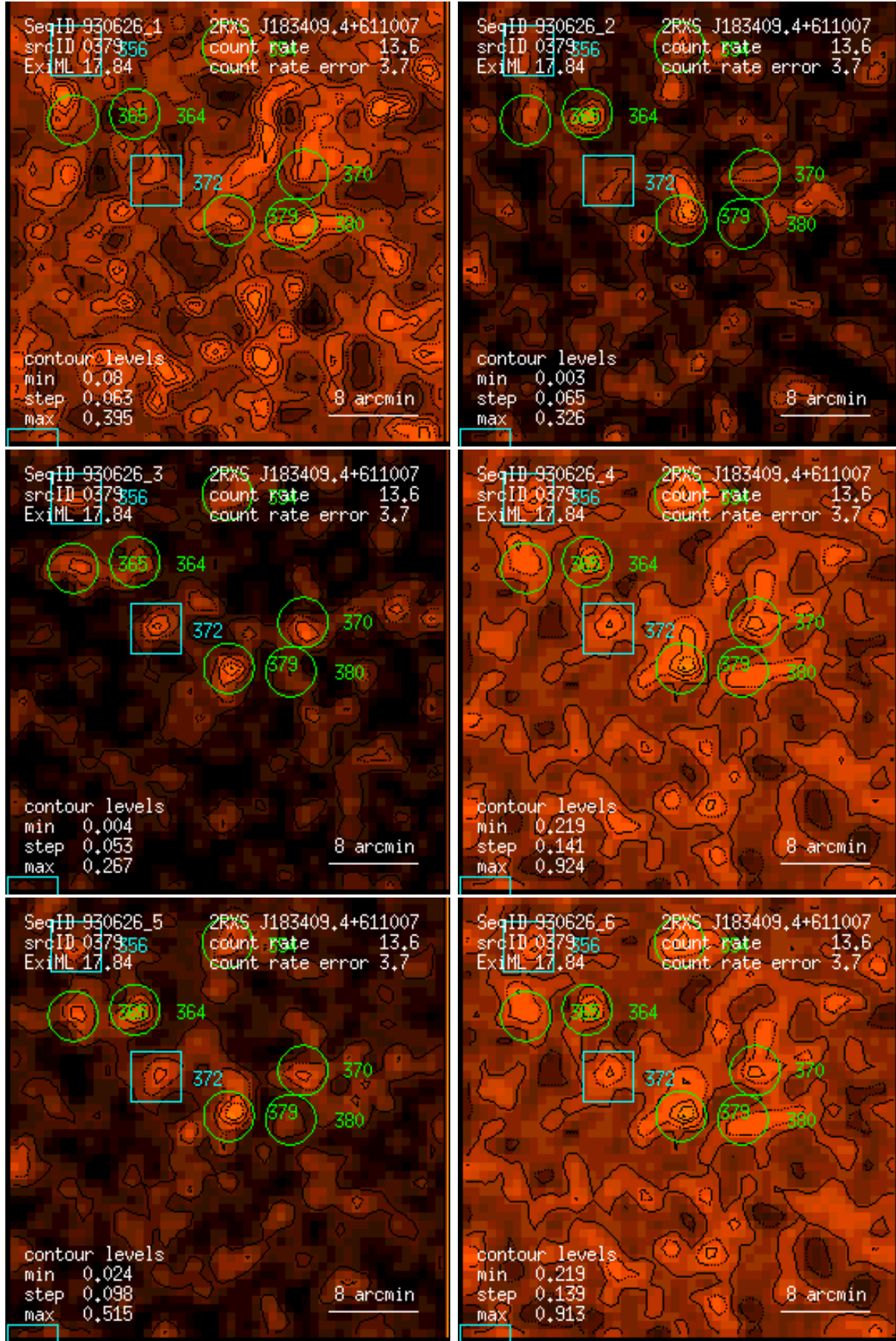
Figure 379: RASS 930626: detection 0379: band rate images, Gaussian filter: (1) PSPC channels 11 – 41, (2) 52 – 90, (3) 91 – 201, (4) 11 – 235, (5) 52 – 201, (6) 11 – 201. Broad band rates in counts/ks. Band rate contour levels in counts/ks/arcmin 2 .
