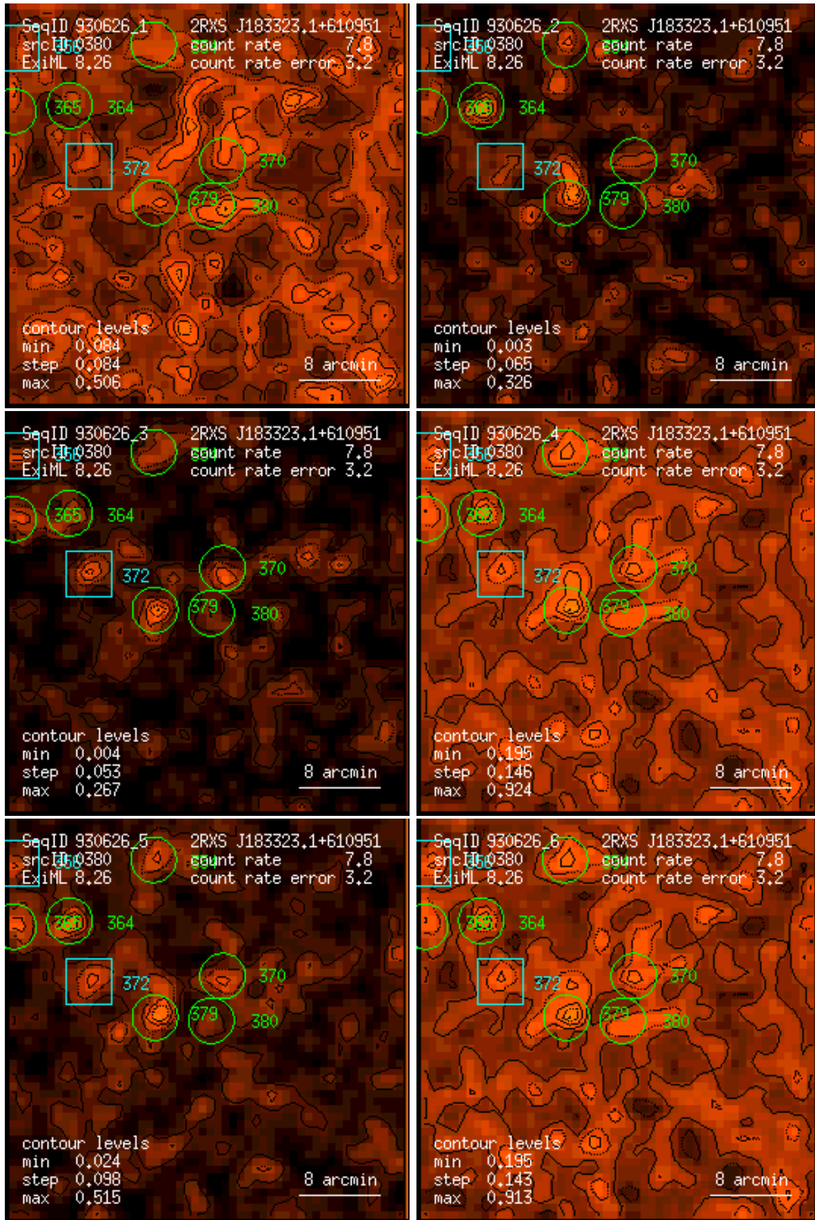
Figure 380: RASS 930626: detection 0380: band rate images, Gaussian filter: (1) PSPC channels 11 – 41, (2) 52 – 90, (3) 91 – 201, (4) 11 – 235, (5) 52 – 201, (6) 11 – 201. Broad band rates in counts/ks. Band rate contour levels in counts/ks/arcmin 2 .
