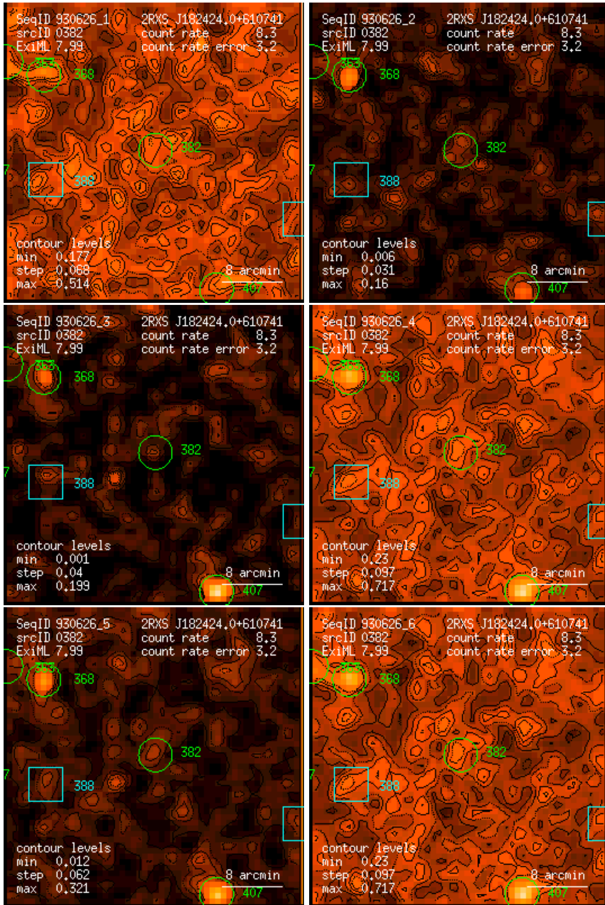
Figure 382: RASS 930626: detection 0382: band rate images, Gaussian filter: (1) PSPC channels 11 – 41, (2) 52 – 90, (3) 91 – 201, (4) 11 – 235, (5) 52 – 201, (6) 11 – 201. Broad band rates in counts/ks. Band rate contour levels in counts/ks/arcmin 2 .
