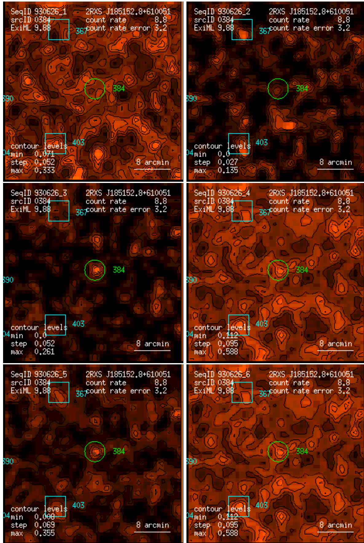
Figure 384: RASS 930626: detection 0384: band rate images, Gaussian filter: (1) PSPC channels 11 – 41, (2) 52 – 90, (3) 91 – 201, (4) 11 – 235, (5) 52 – 201, (6) 11 – 201. Broad band rates in counts/ks. Band rate contour levels in counts/ks/arcmin 2 .
