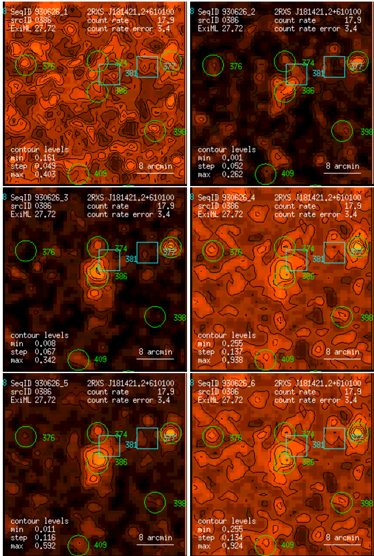
Figure 386: RASS 930626: detection 0386: band rate images, Gaussian filter: (1) PSPC channels 11 – 41, (2) 52 – 90, (3) 91 – 201, (4) 11 – 235, (5) 52 – 201, (6) 11 – 201. Broad band rates in counts/ks. Band rate contour levels in counts/ks/arcmin 2 .
