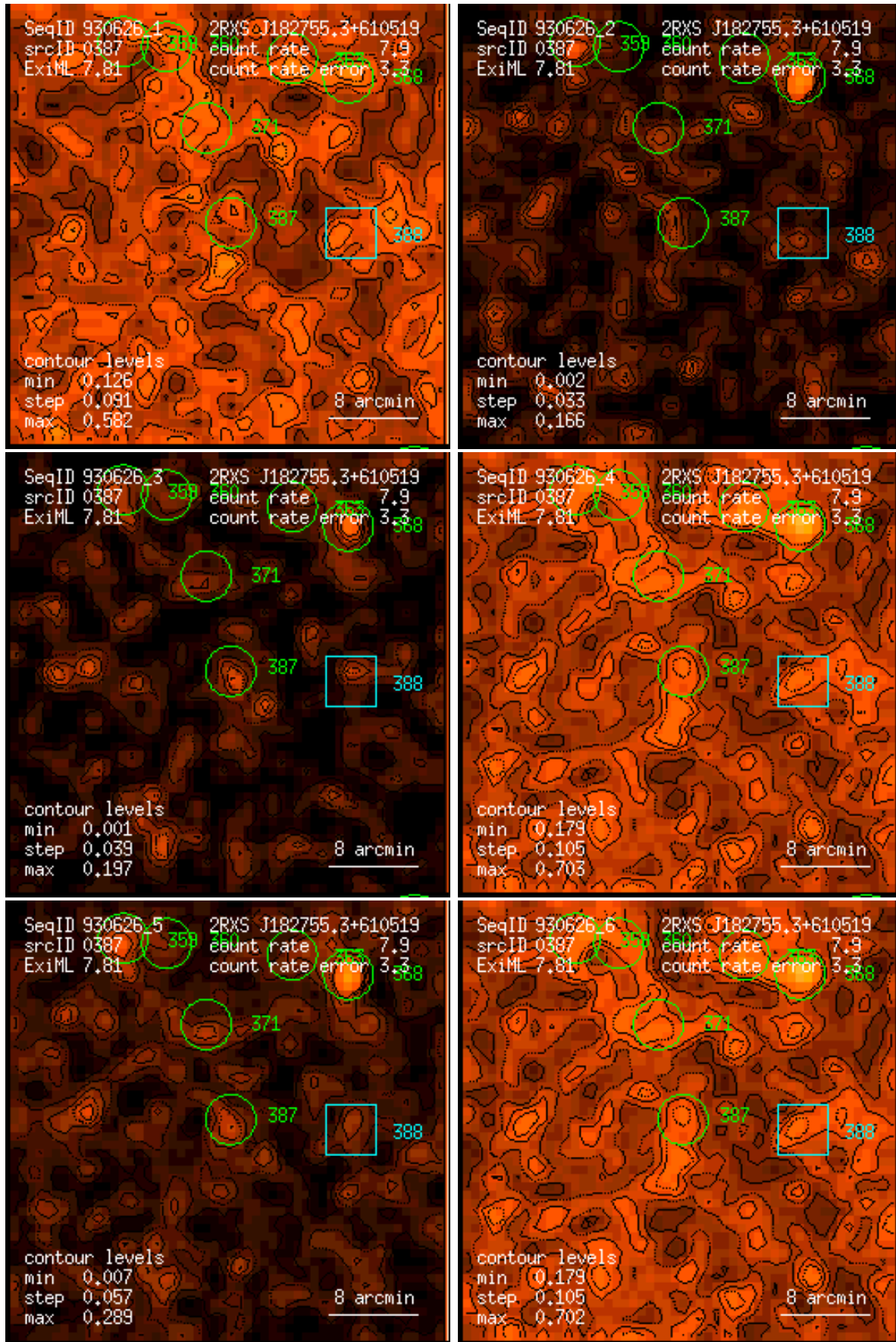
Figure 387: RASS 930626: detection 0387: band rate images, Gaussian filter: (1) PSPC channels 11 – 41, (2) 52 – 90, (3) 91 – 201, (4) 11 – 235, (5) 52 – 201, (6) 11 – 201. Broad band rates in counts/ks. Band rate contour levels in counts/ks/arcmin 2 .
