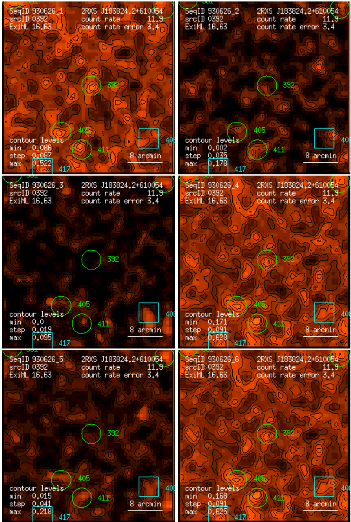
Figure 392: RASS 930626: detection 0392: band rate images, Gaussian filter: (1) PSPC channels 11 – 41, (2) 52 – 90, (3) 91 – 201, (4) 11 – 235, (5) 52 – 201, (6) 11 – 201. Broad band rates in counts/ks. Band rate contour levels in counts/ks/arcmin 2 .
