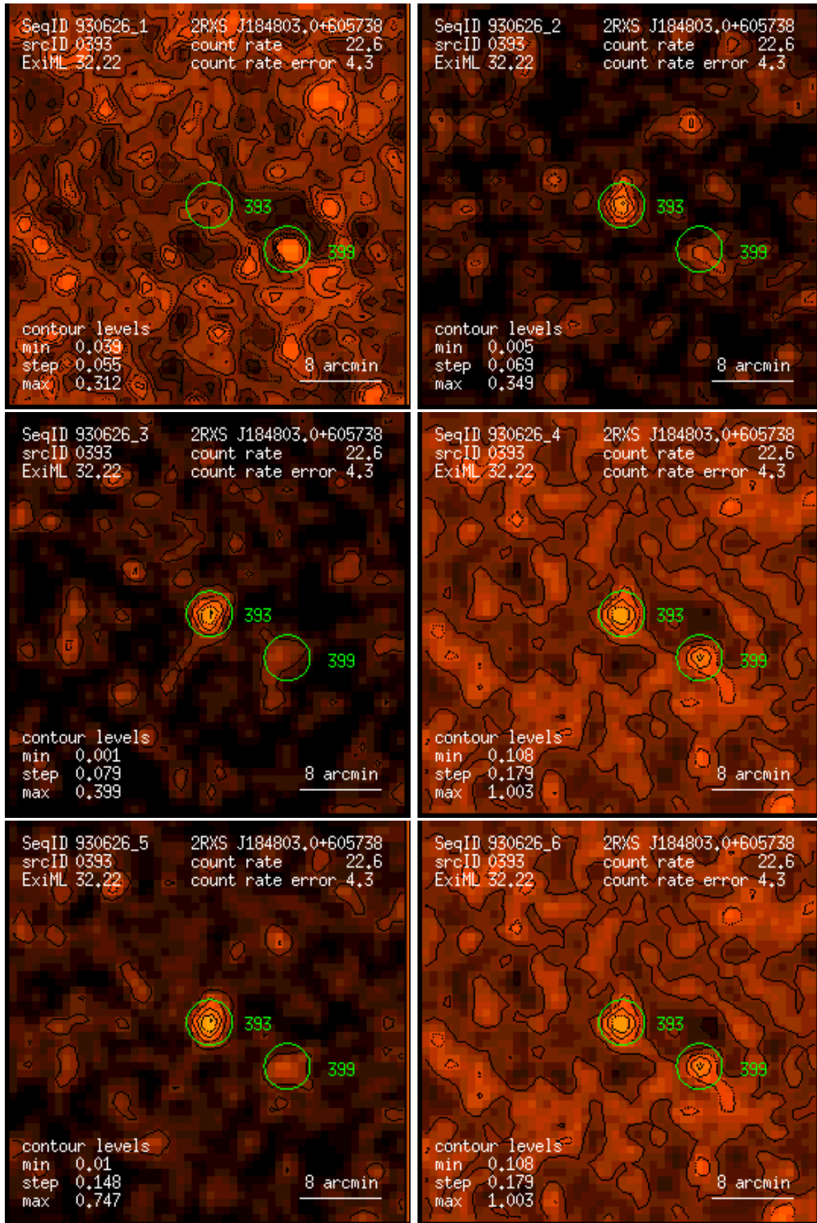
Figure 393: RASS 930626: detection 0393: band rate images, Gaussian filter: (1) PSPC channels 11 – 41, (2) 52 – 90, (3) 91 – 201, (4) 11 – 235, (5) 52 – 201, (6) 11 – 201. Broad band rates in counts/ks. Band rate contour levels in counts/ks/arcmin 2 .
