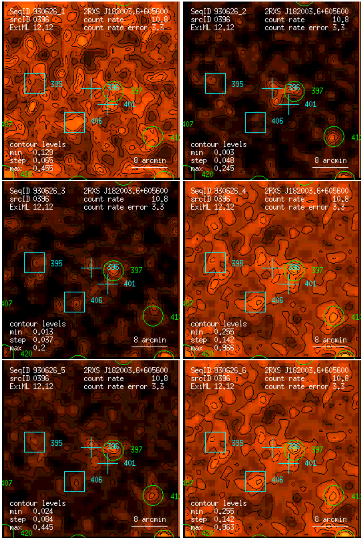
Figure 396: RASS 930626: detection 0396: band rate images, Gaussian filter: (1) PSPC channels 11 – 41, (2) 52 – 90, (3) 91 – 201, (4) 11 – 235, (5) 52 – 201, (6) 11 – 201. Broad band rates in counts/ks. Band rate contour levels in counts/ks/arcmin 2 .
