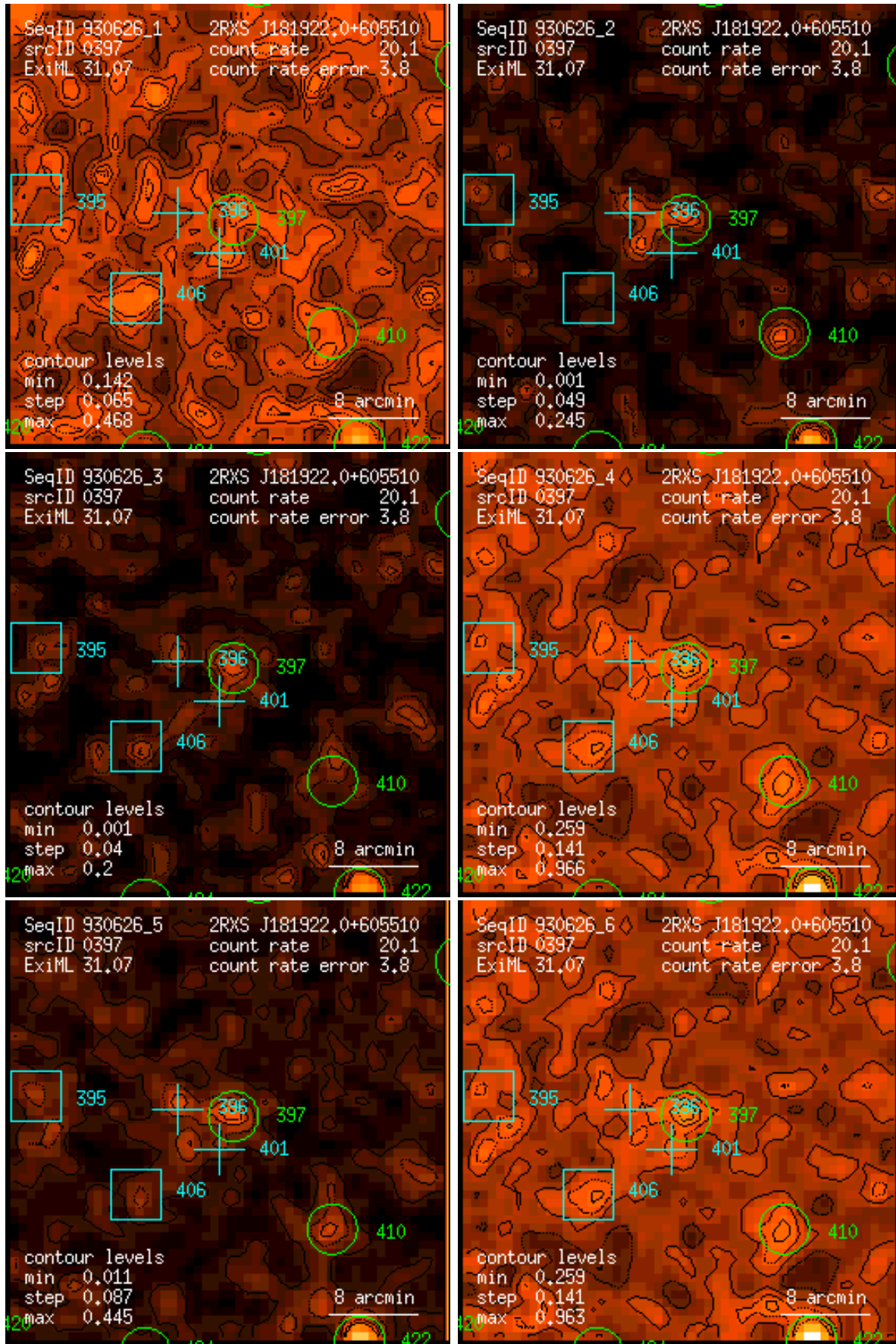
Figure 397: RASS 930626: detection 0397: band rate images, Gaussian filter: (1) PSPC channels 11 – 41, (2) 52 – 90, (3) 91 – 201, (4) 11 – 235, (5) 52 – 201, (6) 11 – 201. Broad band rates in counts/ks. Band rate contour levels in counts/ks/arcmin 2 .
