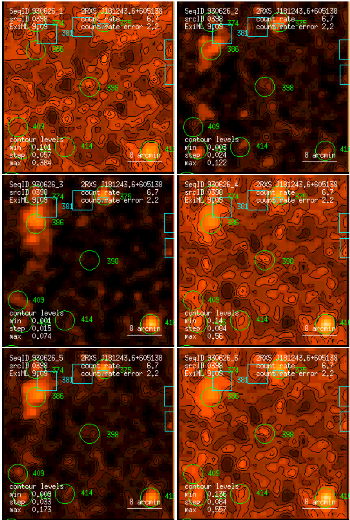
Figure 398: RASS 930626: detection 0398: band rate images, Gaussian filter: (1) PSPC channels 11 – 41, (2) 52 – 90, (3) 91 – 201, (4) 11 – 235, (5) 52 – 201, (6) 11 – 201. Broad band rates in counts/ks. Band rate contour levels in counts/ks/arcmin 2 .
