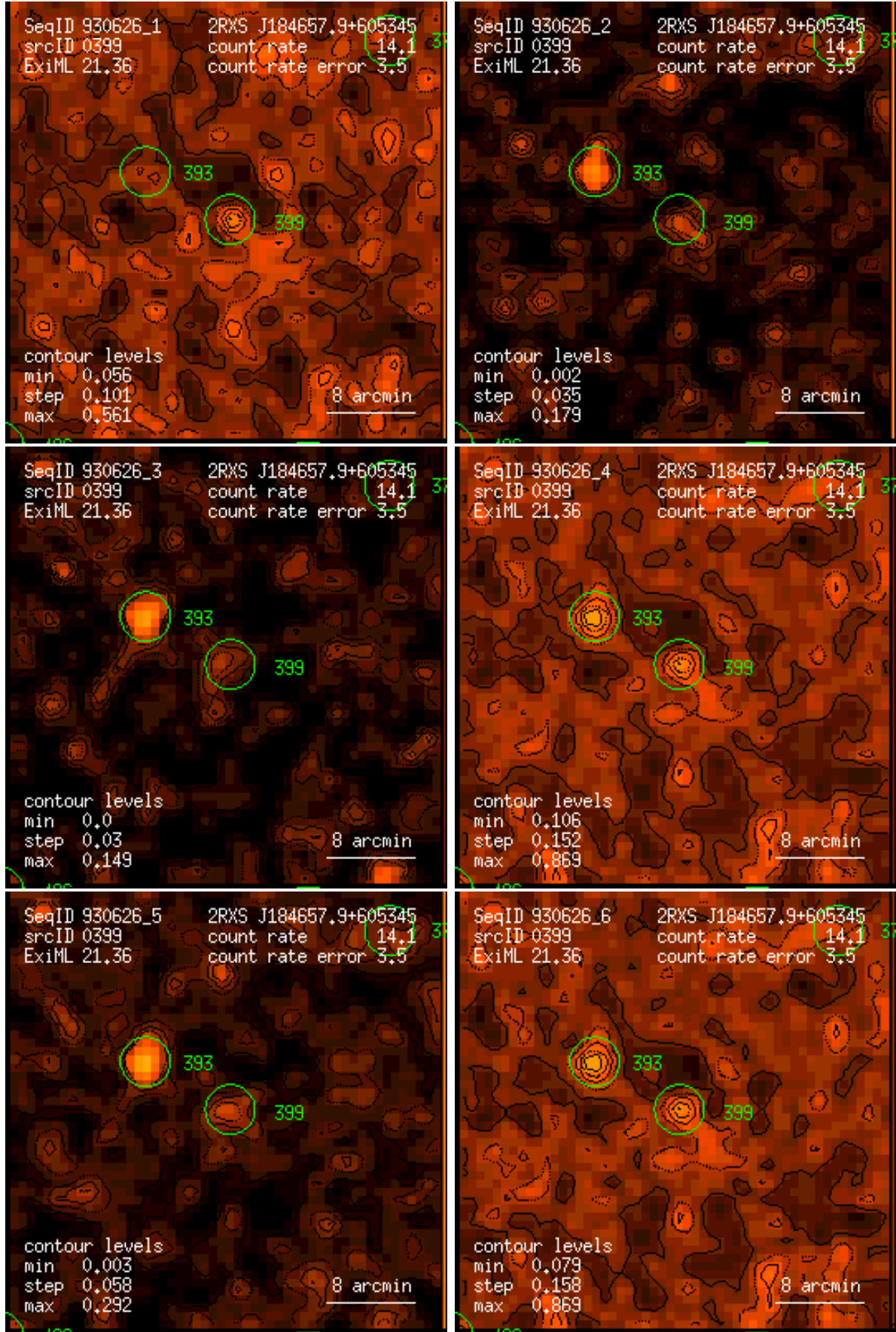
Figure 399: RASS 930626: detection 0399: band rate images, Gaussian filter: (1) PSPC channels 11 – 41, (2) 52 – 90, (3) 91 – 201, (4) 11 – 235, (5) 52 – 201, (6) 11 – 201. Broad band rates in counts/ks. Band rate contour levels in counts/ks/arcmin 2 .
