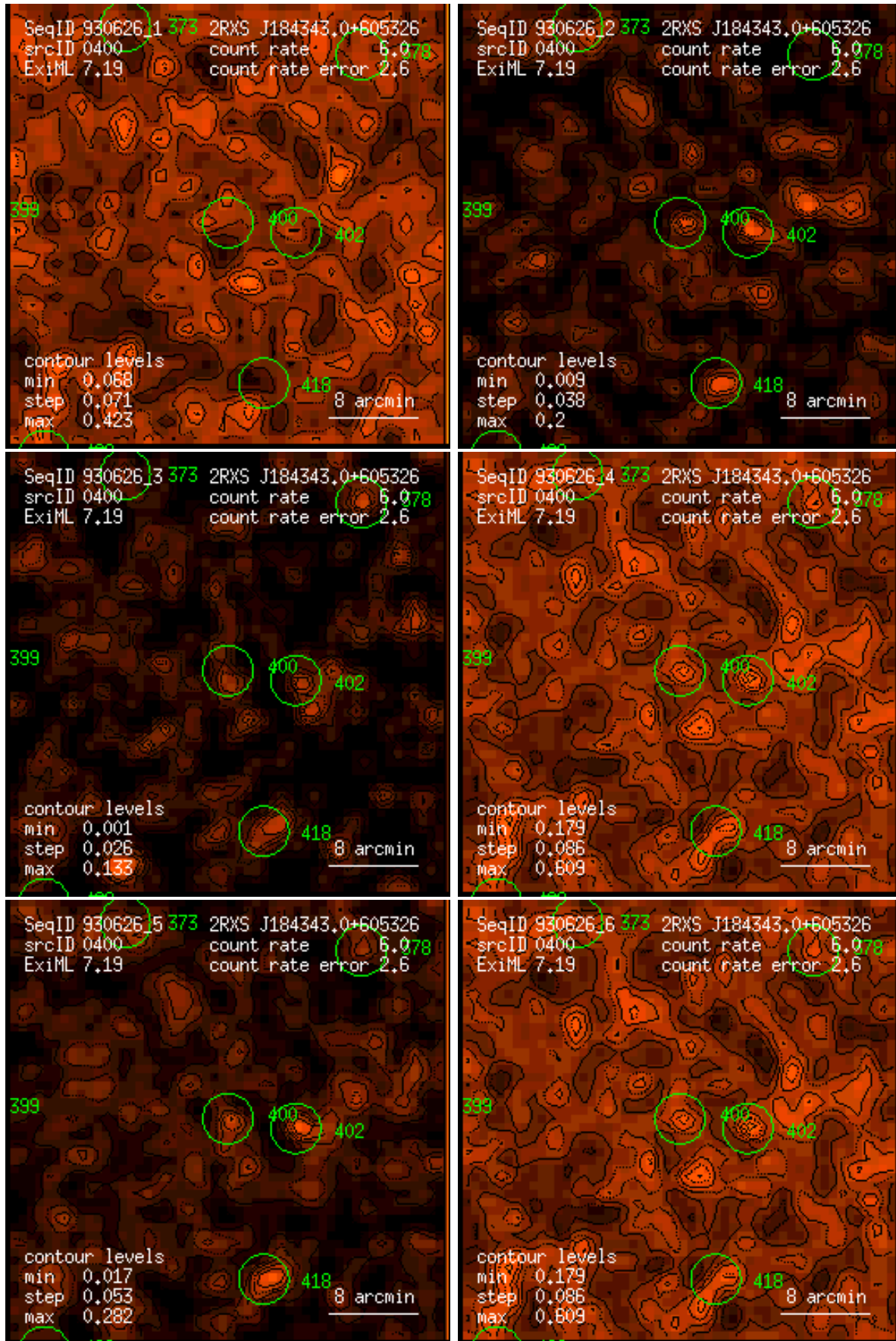
Figure 400: RASS 930626: detection 0400: band rate images, Gaussian filter: (1) PSPC channels 11 – 41, (2) 52 – 90, (3) 91 – 201, (4) 11 – 235, (5) 52 – 201, (6) 11 – 201. Broad band rates in counts/ks. Band rate contour levels in counts/ks/arcmin 2 .
