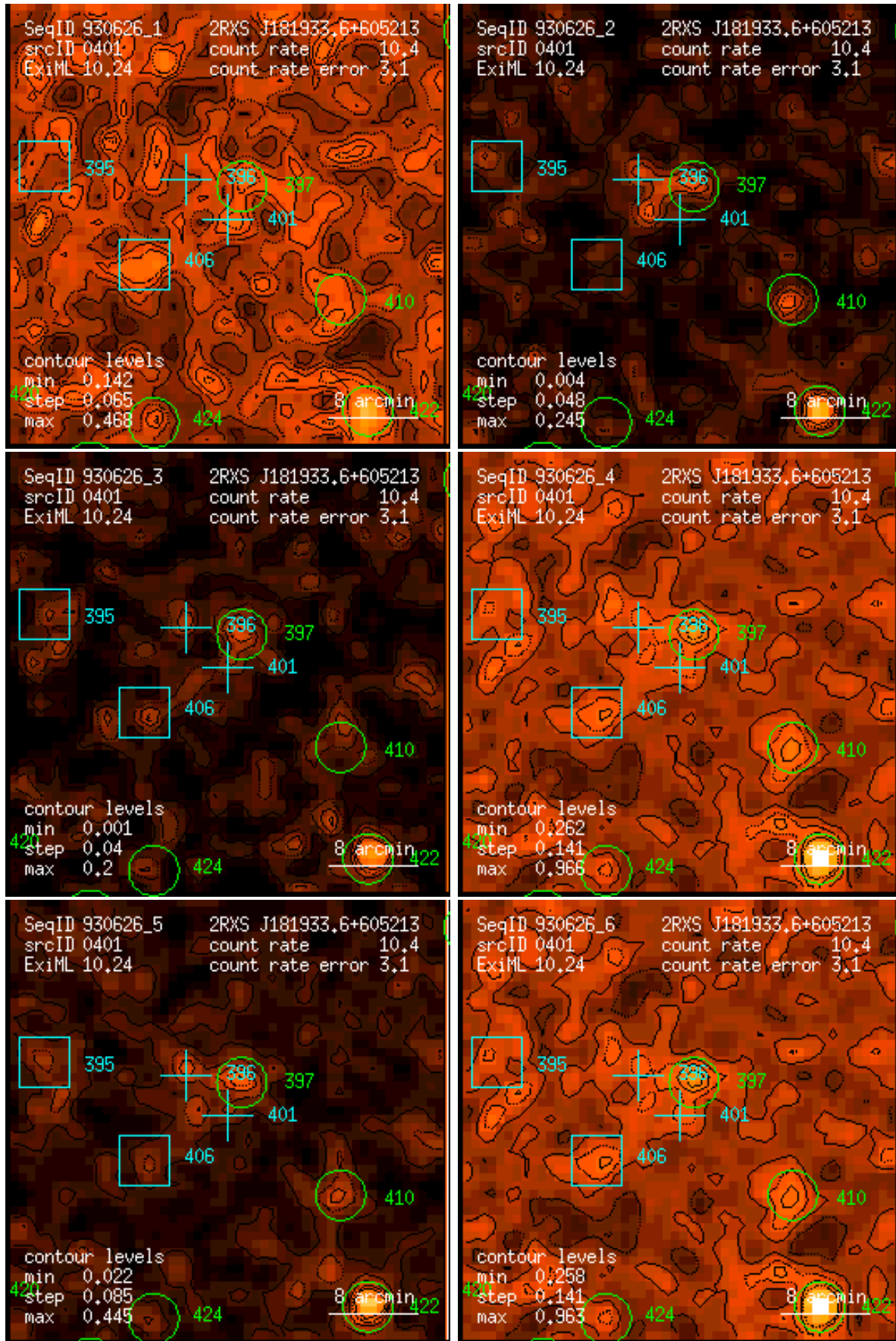
Figure 401: RASS 930626: detection 0401: band rate images, Gaussian filter: (1) PSPC channels 11 – 41, (2) 52 – 90, (3) 91 – 201, (4) 11 – 235, (5) 52 – 201, (6) 11 – 201. Broad band rates in counts/ks. Band rate contour levels in counts/ks/arcmin 2 .
