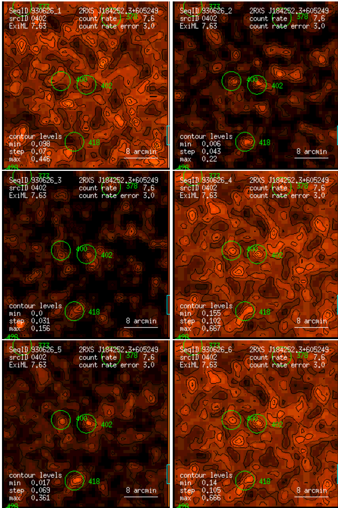
Figure 402: RASS 930626: detection 0402: band rate images, Gaussian filter: (1) PSPC channels 11 – 41, (2) 52 – 90, (3) 91 – 201, (4) 11 – 235, (5) 52 – 201, (6) 11 – 201. Broad band rates in counts/ks. Band rate contour levels in counts/ks/arcmin 2 .
