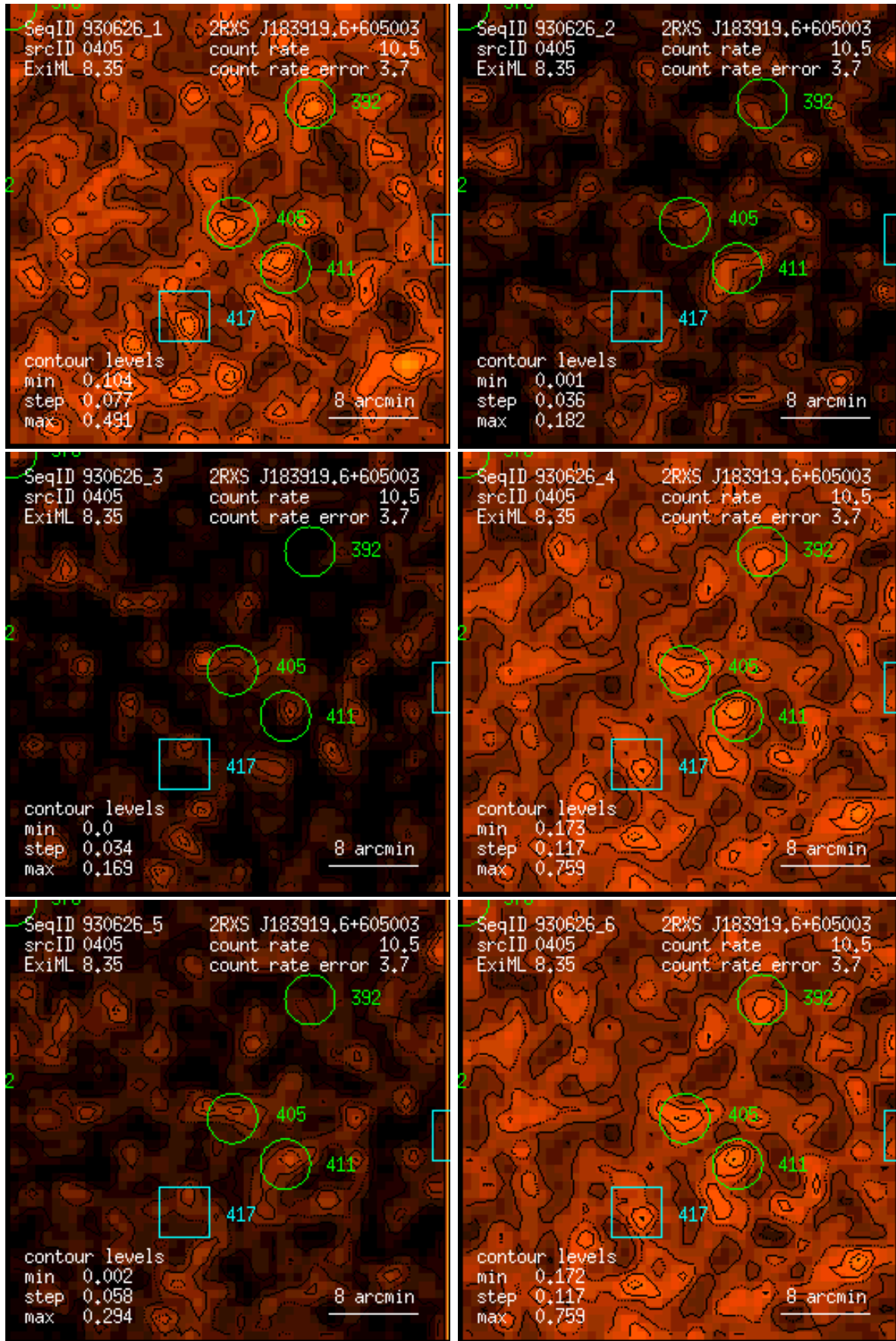
Figure 405: RASS 930626: detection 0405: band rate images, Gaussian filter: (1) PSPC channels 11 – 41, (2) 52 – 90, (3) 91 – 201, (4) 11 – 235, (5) 52 – 201, (6) 11 – 201. Broad band rates in counts/ks. Band rate contour levels in counts/ks/arcmin 2 .
