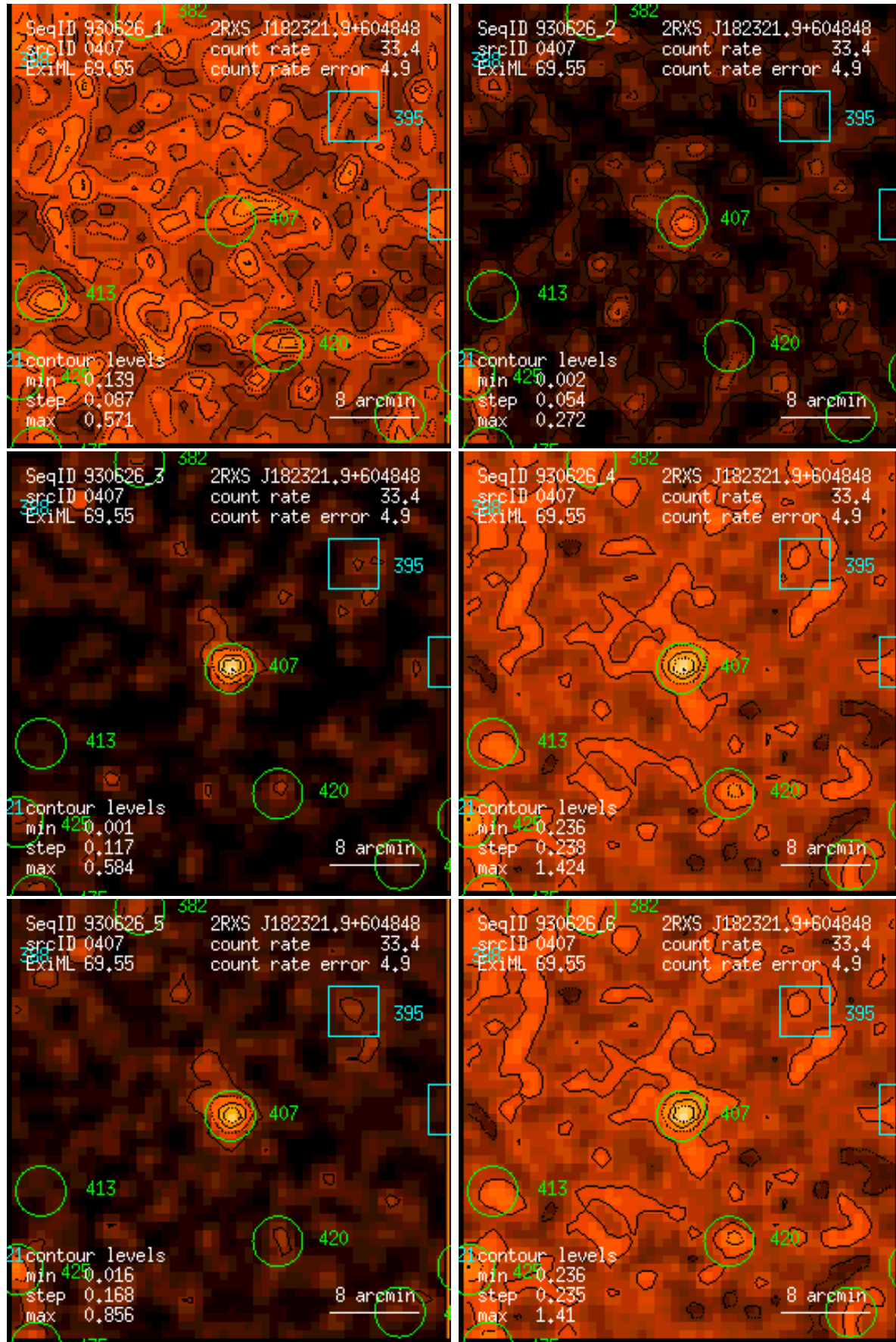
Figure 407: RASS 930626: detection 0407: band rate images, Gaussian filter: (1) PSPC channels 11 – 41, (2) 52 – 90, (3) 91 – 201, (4) 11 – 235, (5) 52 – 201, (6) 11 – 201. Broad band rates in counts/ks. Band rate contour levels in counts/ks/arcmin 2 .
