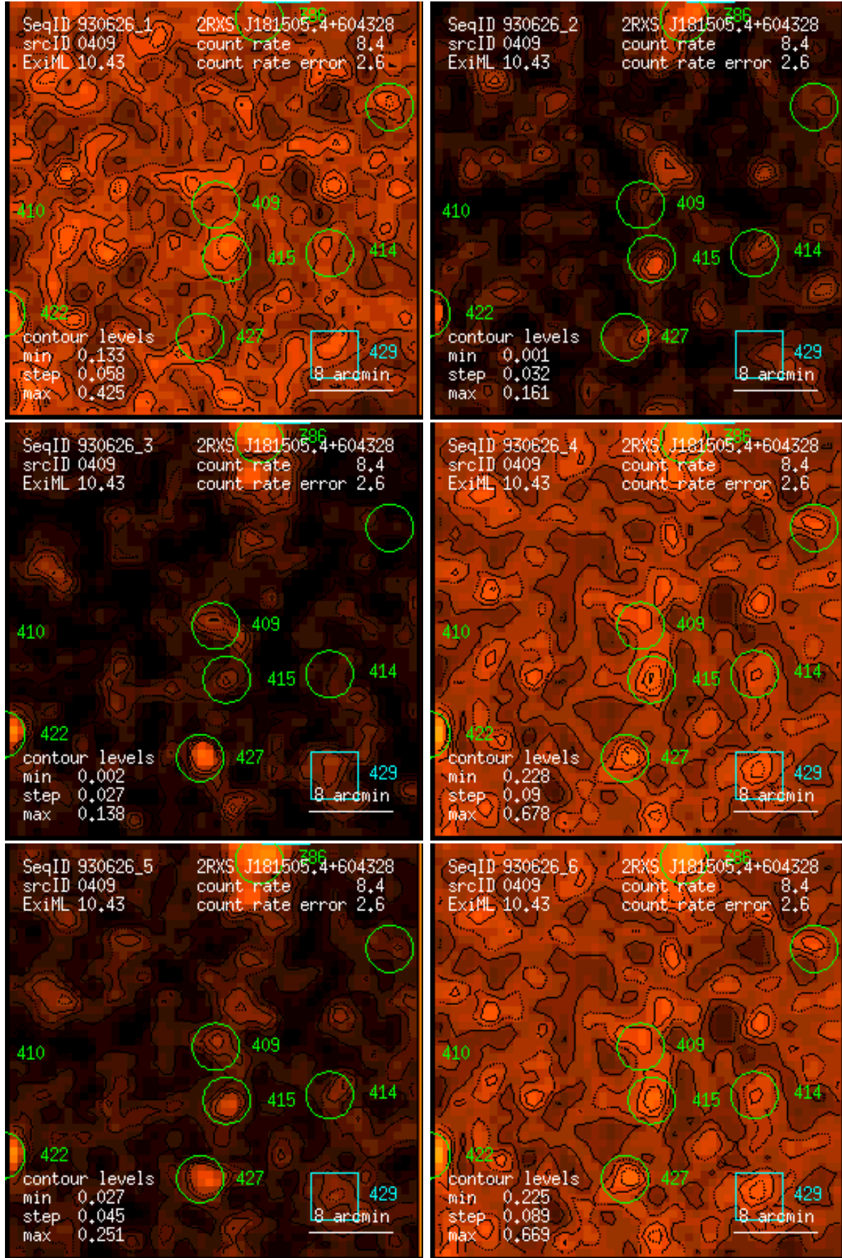
Figure 409: RASS 930626: detection 0409: band rate images, Gaussian filter: (1) PSPC channels 11 – 41, (2) 52 – 90, (3) 91 – 201, (4) 11 – 235, (5) 52 – 201, (6) 11 – 201. Broad band rates in counts/ks. Band rate contour levels in counts/ks/arcmin 2 .
