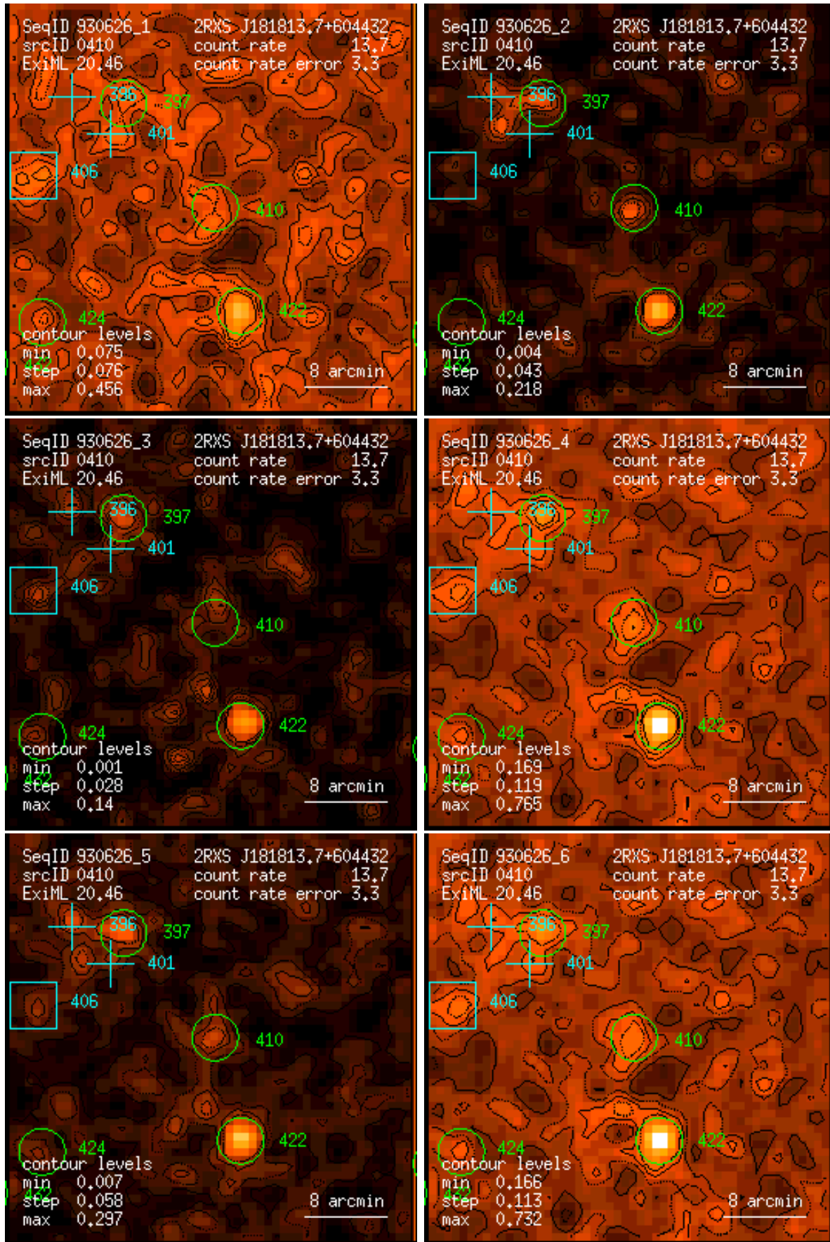
Figure 410: RASS 930626: detection 0410: band rate images, Gaussian filter: (1) PSPC channels 11 – 41, (2) 52 – 90, (3) 91 – 201, (4) 11 – 235, (5) 52 – 201, (6) 11 – 201. Broad band rates in counts/ks. Band rate contour levels in counts/ks/arcmin 2 .
