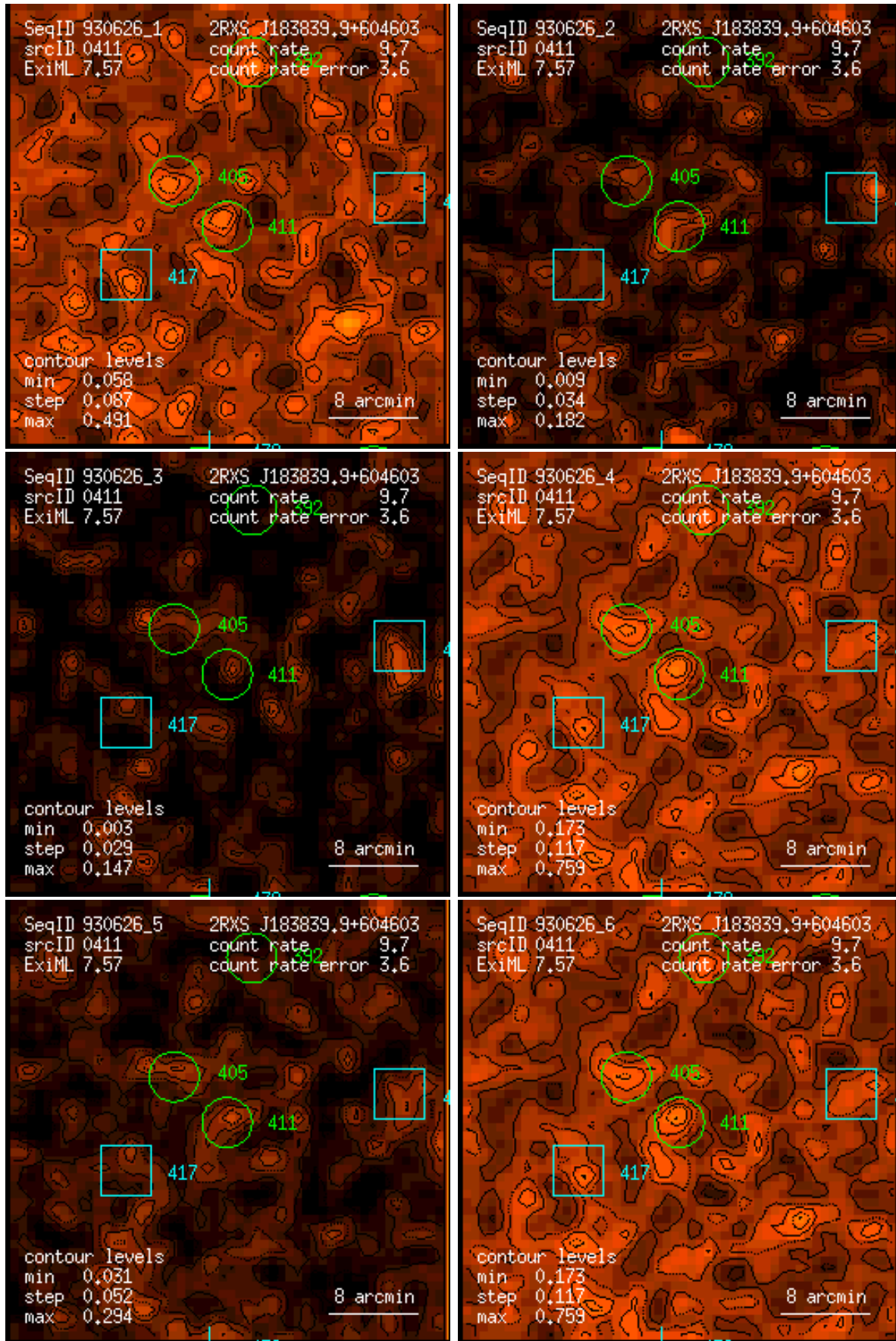
Figure 411: RASS 930626: detection 0411: band rate images, Gaussian filter: (1) PSPC channels 11 – 41, (2) 52 – 90, (3) 91 – 201, (4) 11 – 235, (5) 52 – 201, (6) 11 – 201. Broad band rates in counts/ks. Band rate contour levels in counts/ks/arcmin 2 .
