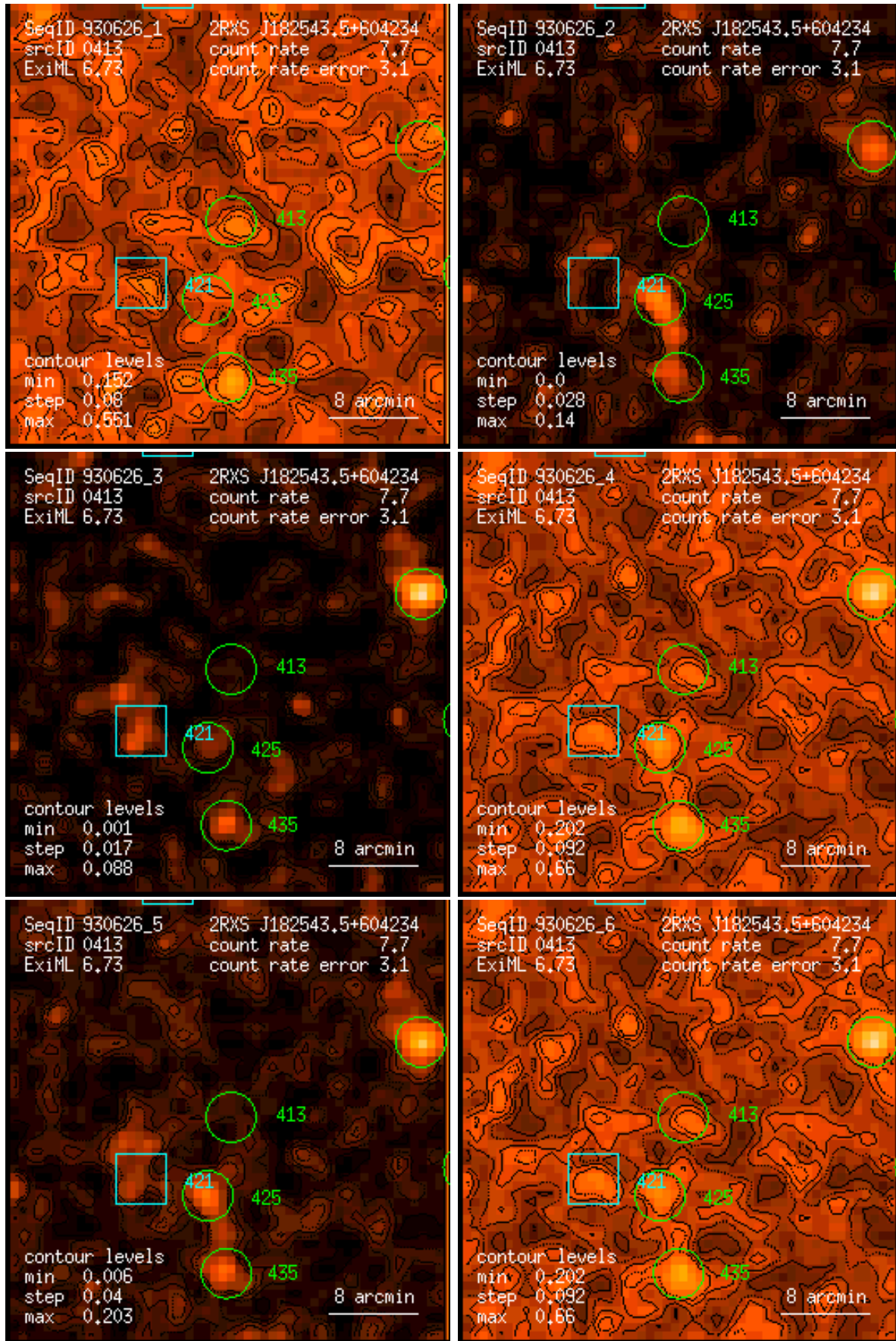
Figure 413: RASS 930626: detection 0413: band rate images, Gaussian filter: (1) PSPC channels 11 – 41, (2) 52 – 90, (3) 91 – 201, (4) 11 – 235, (5) 52 – 201, (6) 11 – 201. Broad band rates in counts/ks. Band rate contour levels in counts/ks/arcmin 2 .
