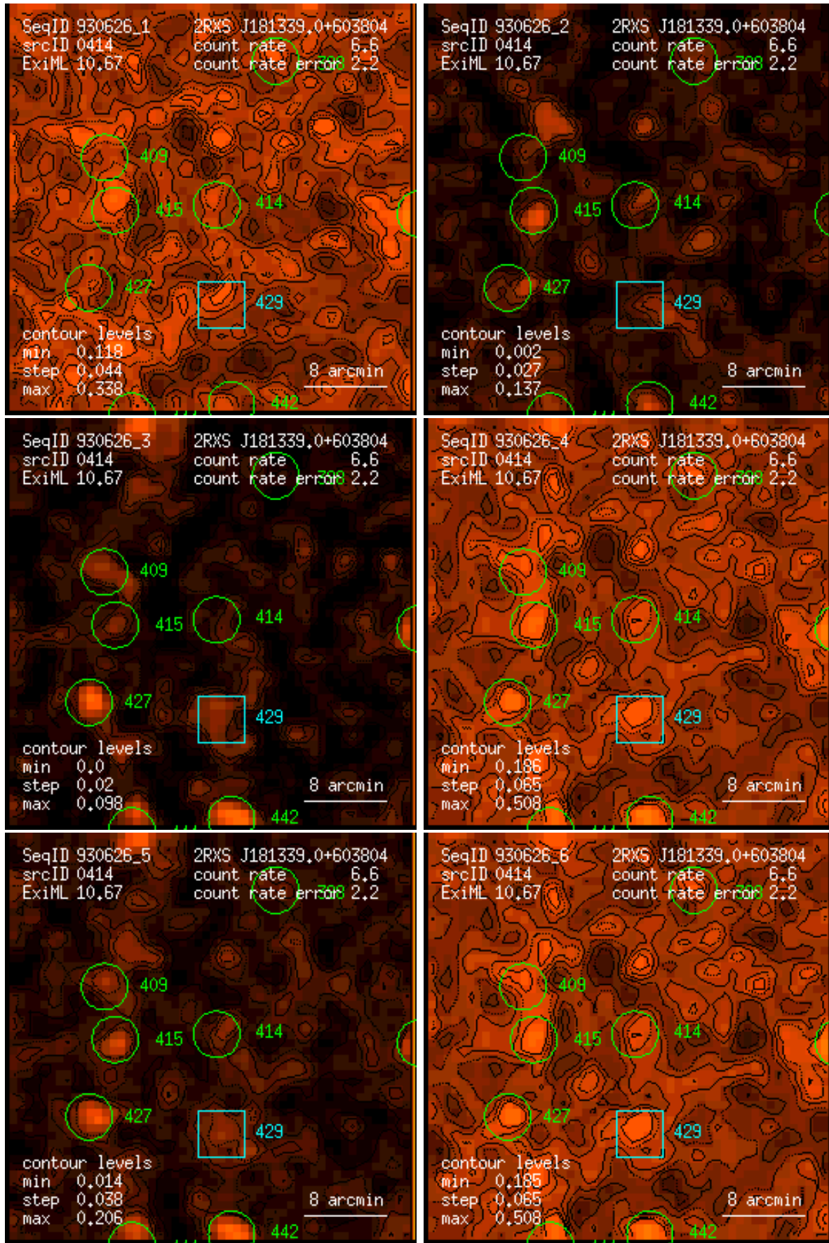
Figure 414: RASS 930626: detection 0414: band rate images, Gaussian filter: (1) PSPC channels 11 – 41, (2) 52 – 90, (3) 91 – 201, (4) 11 – 235, (5) 52 – 201, (6) 11 – 201. Broad band rates in counts/ks. Band rate contour levels in counts/ks/arcmin 2 .
