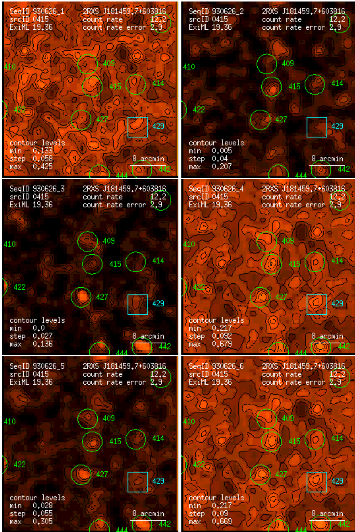
Figure 415: RASS 930626: detection 0415: band rate images, Gaussian filter: (1) PSPC channels 11 – 41, (2) 52 – 90, (3) 91 – 201, (4) 11 – 235, (5) 52 – 201, (6) 11 – 201. Broad band rates in counts/ks. Band rate contour levels in counts/ks/arcmin 2 .
