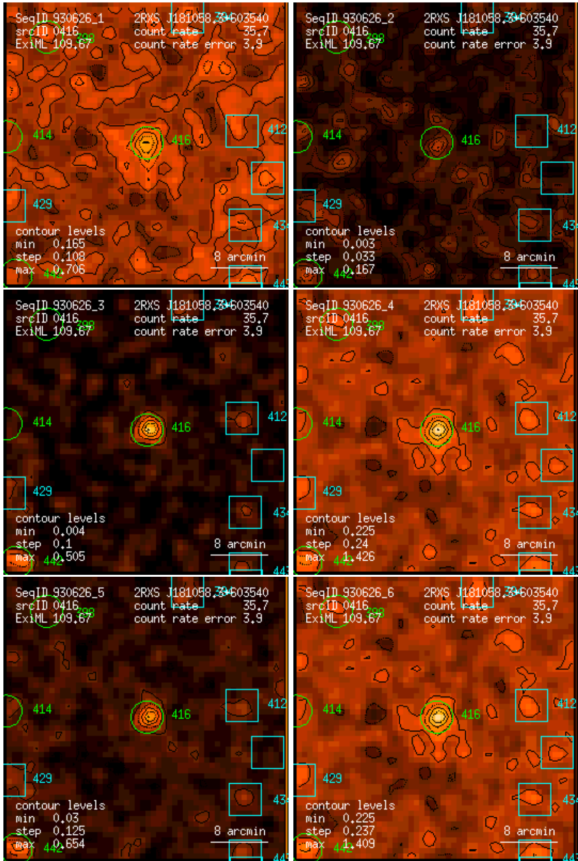
Figure 416: RASS 930626: detection 0416: band rate images, Gaussian filter: (1) PSPC channels 11 – 41, (2) 52 – 90, (3) 91 – 201, (4) 11 – 235, (5) 52 – 201, (6) 11 – 201. Broad band rates in counts/ks. Band rate contour levels in counts/ks/arcmin 2 .
