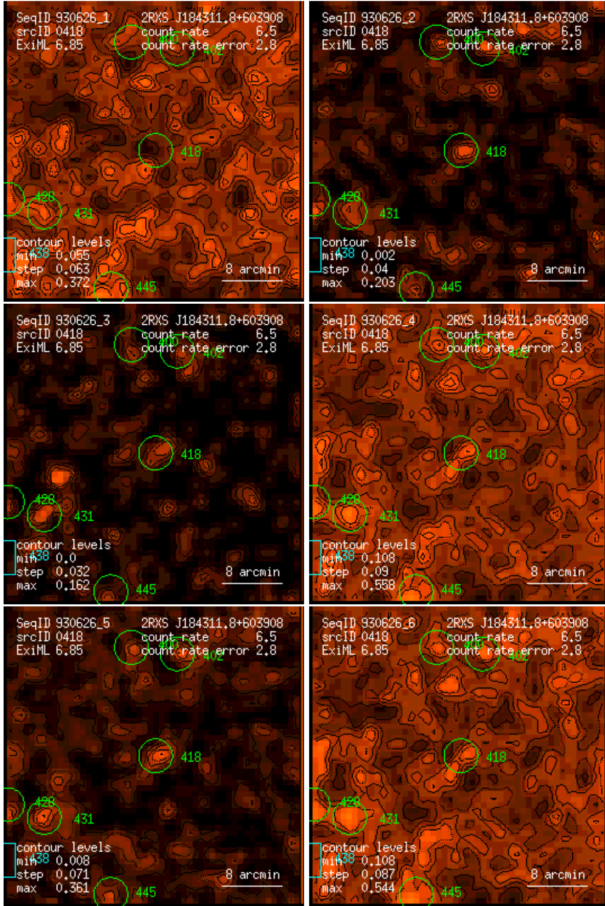
Figure 418: RASS 930626: detection 0418: band rate images, Gaussian filter: (1) PSPC channels 11 – 41, (2) 52 – 90, (3) 91 – 201, (4) 11 – 235, (5) 52 – 201, (6) 11 – 201. Broad band rates in counts/ks. Band rate contour levels in counts/ks/arcmin 2 .
