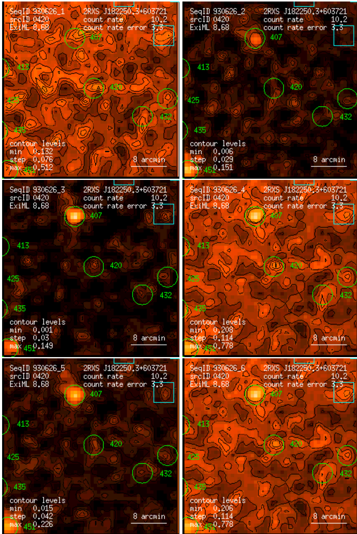
Figure 420: RASS 930626: detection 0420: band rate images, Gaussian filter: (1) PSPC channels 11 – 41, (2) 52 – 90, (3) 91 – 201, (4) 11 – 235, (5) 52 – 201, (6) 11 – 201. Broad band rates in counts/ks. Band rate contour levels in counts/ks/arcmin 2 .
