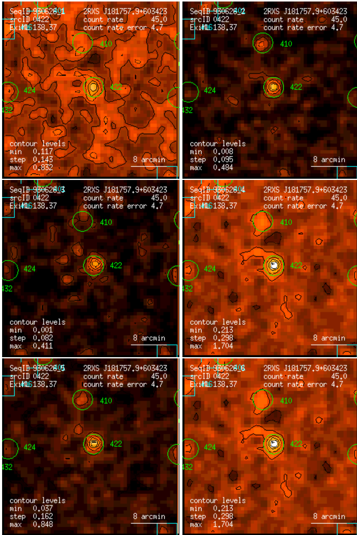
Figure 422: RASS 930626: detection 0422: band rate images, Gaussian filter: (1) PSPC channels 11 – 41, (2) 52 – 90, (3) 91 – 201, (4) 11 – 235, (5) 52 – 201, (6) 11 – 201. Broad band rates in counts/ks. Band rate contour levels in counts/ks/arcmin 2 .
