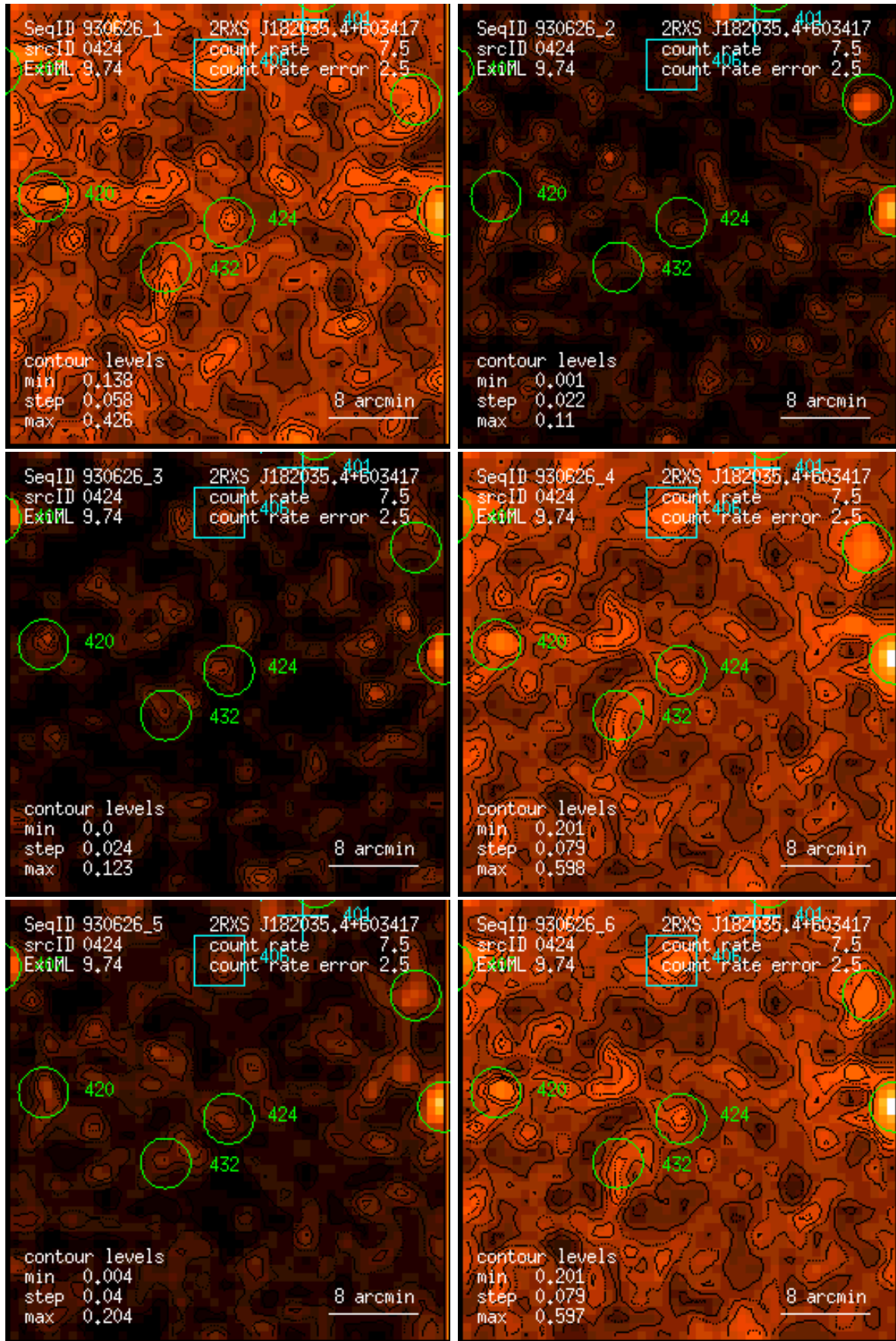
Figure 424: RASS 930626: detection 0424: band rate images, Gaussian filter: (1) PSPC channels 11 – 41, (2) 52 – 90, (3) 91 – 201, (4) 11 – 235, (5) 52 – 201, (6) 11 – 201. Broad band rates in counts/ks. Band rate contour levels in counts/ks/arcmin 2 .
