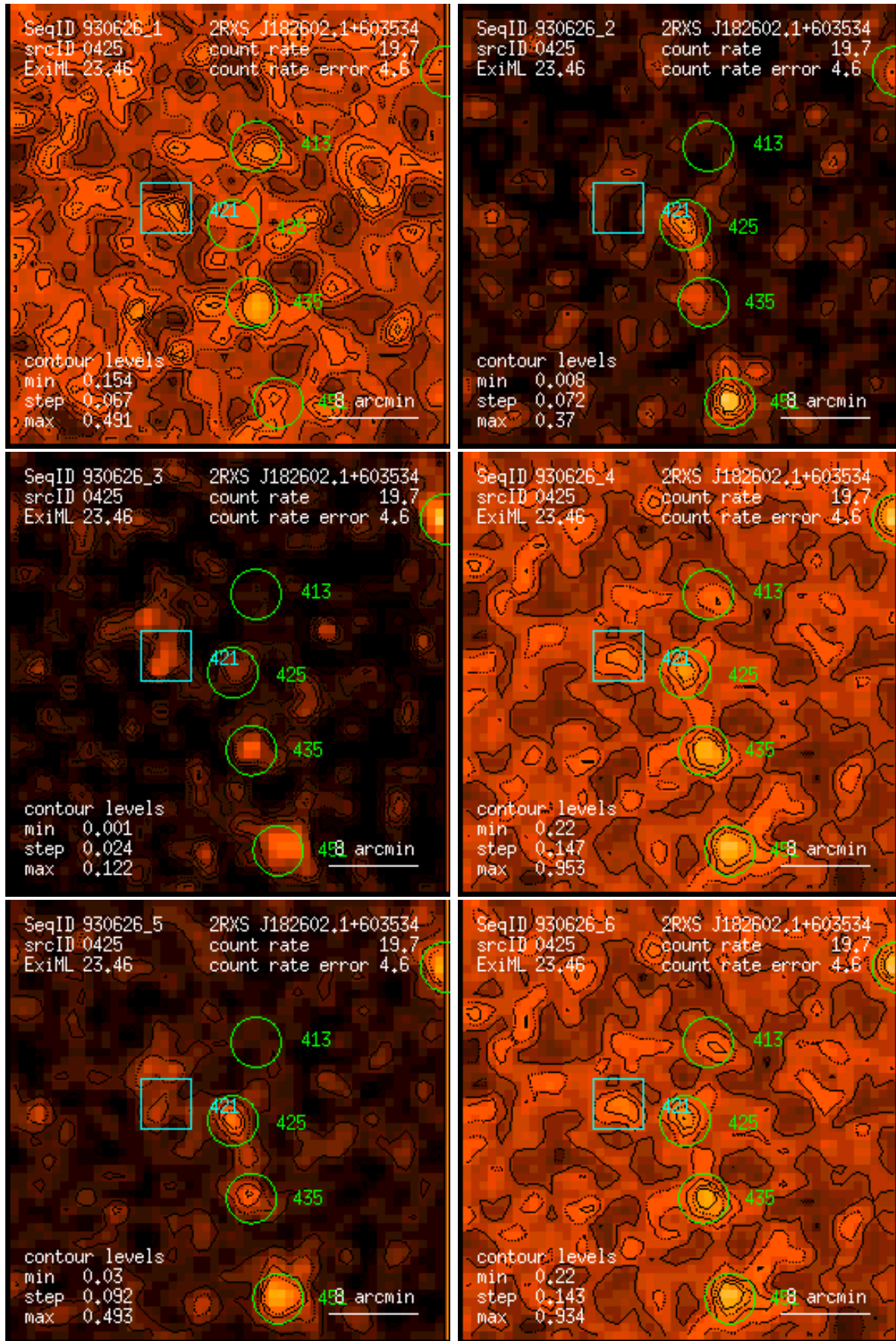
Figure 425: RASS 930626: detection 0425: band rate images, Gaussian filter: (1) PSPC channels 11 – 41, (2) 52 – 90, (3) 91 – 201, (4) 11 – 235, (5) 52 – 201, (6) 11 – 201. Broad band rates in counts/ks. Band rate contour levels in counts/ks/arcmin 2 .
