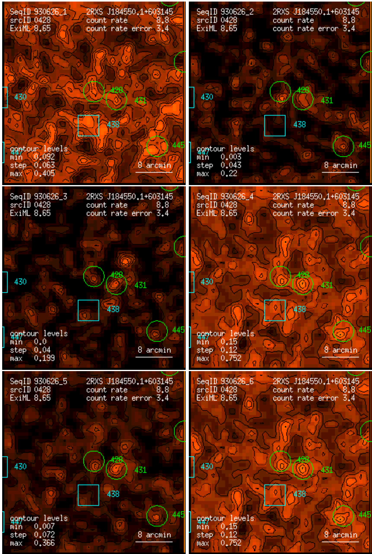
Figure 428: RASS 930626: detection 0428: band rate images, Gaussian filter: (1) PSPC channels 11 – 41, (2) 52 – 90, (3) 91 – 201, (4) 11 – 235, (5) 52 – 201, (6) 11 – 201. Broad band rates in counts/ks. Band rate contour levels in counts/ks/arcmin 2 .
