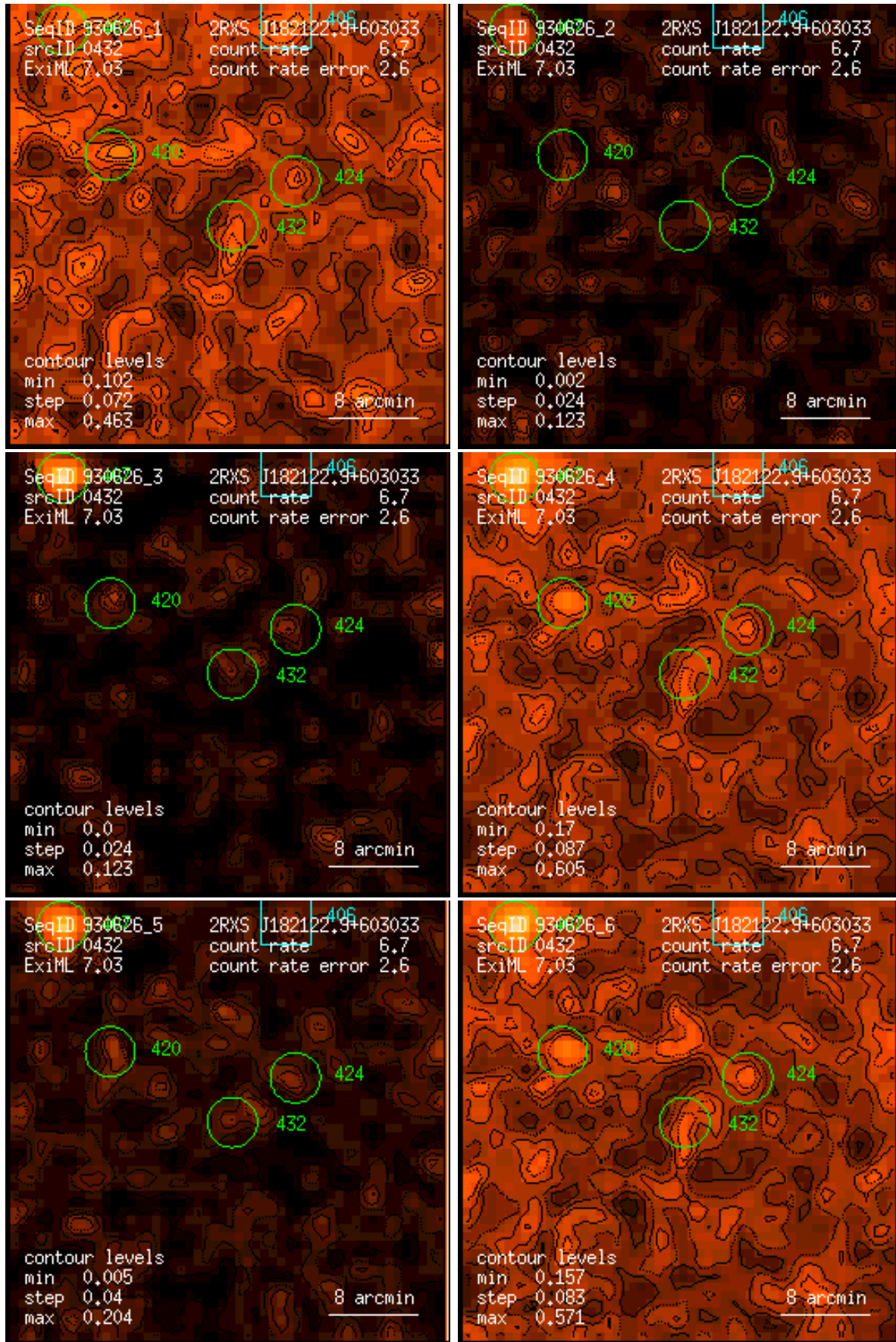
Figure 432: RASS 930626: detection 0432: band rate images, Gaussian filter: (1) PSPC channels 11 – 41, (2) 52 – 90, (3) 91 – 201, (4) 11 – 235, (5) 52 – 201, (6) 11 – 201. Broad band rates in counts/ks. Band rate contour levels in counts/ks/arcmin 2 .
