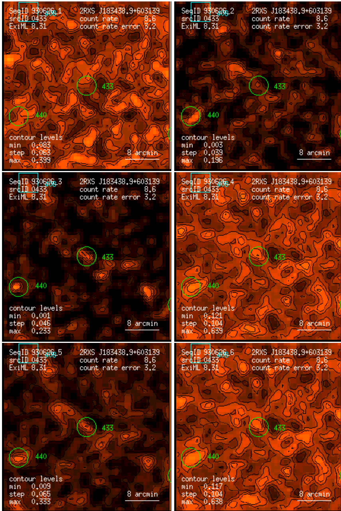
Figure 433: RASS 930626: detection 0433: band rate images, Gaussian filter: (1) PSPC channels 11 – 41, (2) 52 – 90, (3) 91 – 201, (4) 11 – 235, (5) 52 – 201, (6) 11 – 201. Broad band rates in counts/ks. Band rate contour levels in counts/ks/arcmin 2 .
