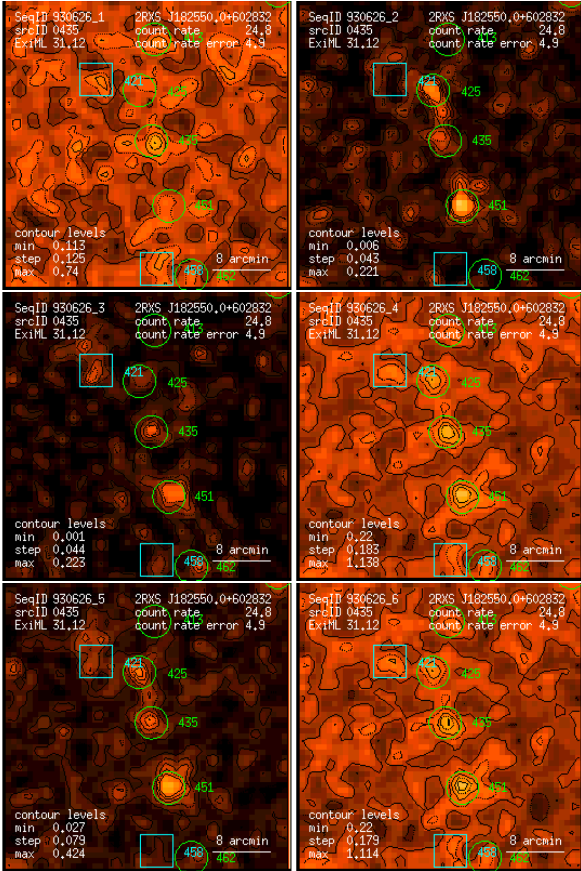
Figure 435: RASS 930626: detection 0435: band rate images, Gaussian filter: (1) PSPC channels 11 – 41, (2) 52 – 90, (3) 91 – 201, (4) 11 – 235, (5) 52 – 201, (6) 11 – 201. Broad band rates in counts/ks. Band rate contour levels in counts/ks/arcmin 2 .
