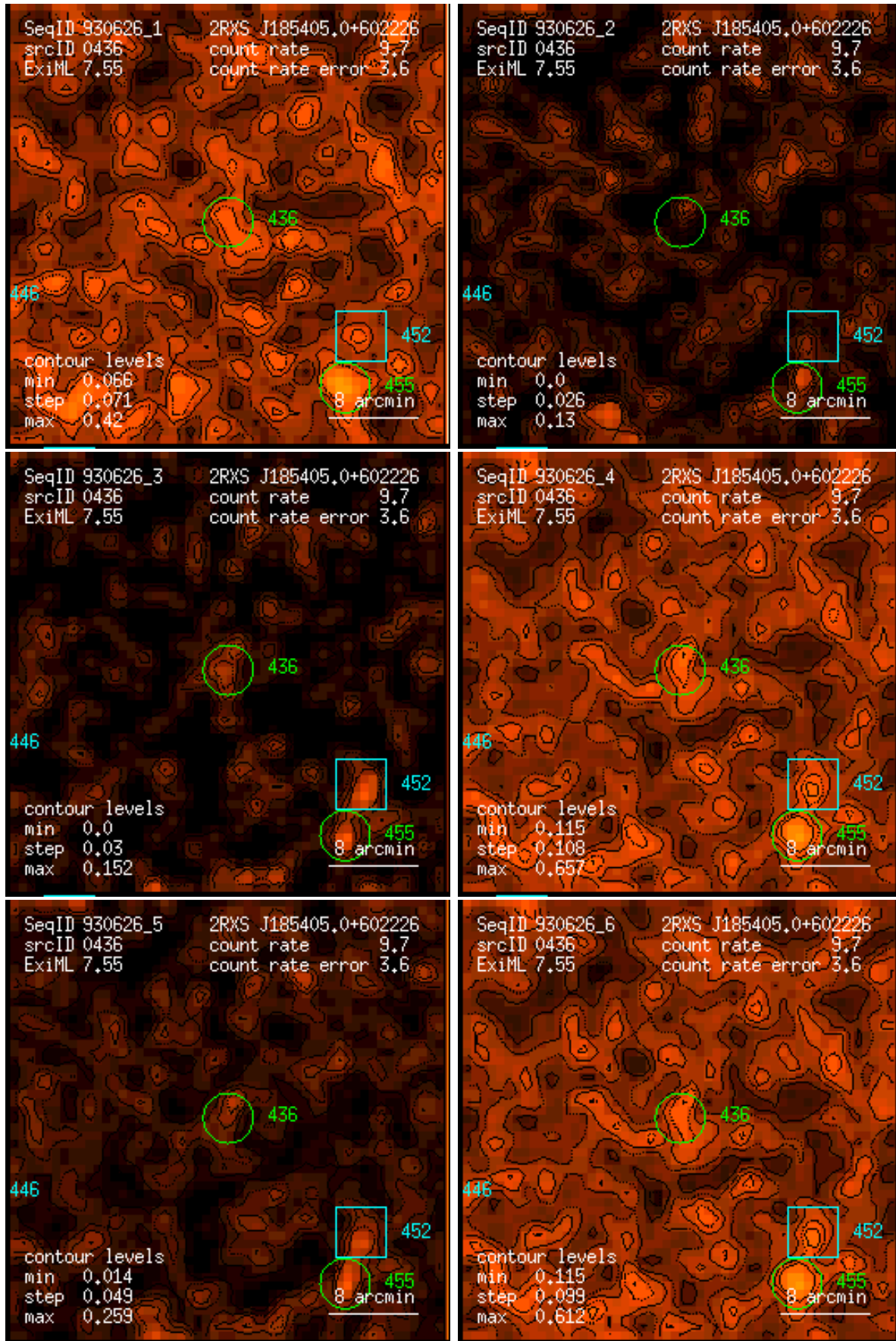
Figure 436: RASS 930626: detection 0436: band rate images, Gaussian filter: (1) PSPC channels 11 – 41, (2) 52 – 90, (3) 91 – 201, (4) 11 – 235, (5) 52 – 201, (6) 11 – 201. Broad band rates in counts/ks. Band rate contour levels in counts/ks/arcmin 2 .
