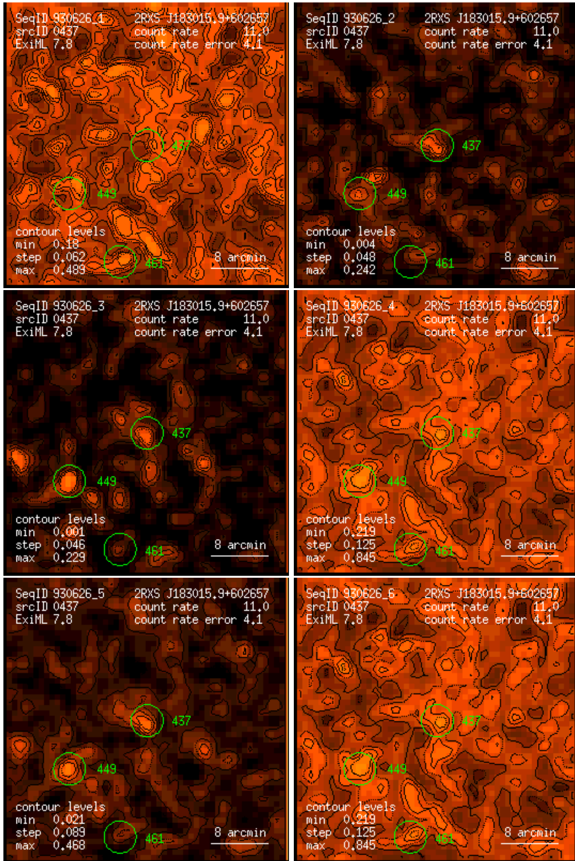
Figure 437: RASS 930626: detection 0437: band rate images, Gaussian filter: (1) PSPC channels 11 – 41, (2) 52 – 90, (3) 91 – 201, (4) 11 – 235, (5) 52 – 201, (6) 11 – 201. Broad band rates in counts/ks. Band rate contour levels in counts/ks/arcmin 2 .
