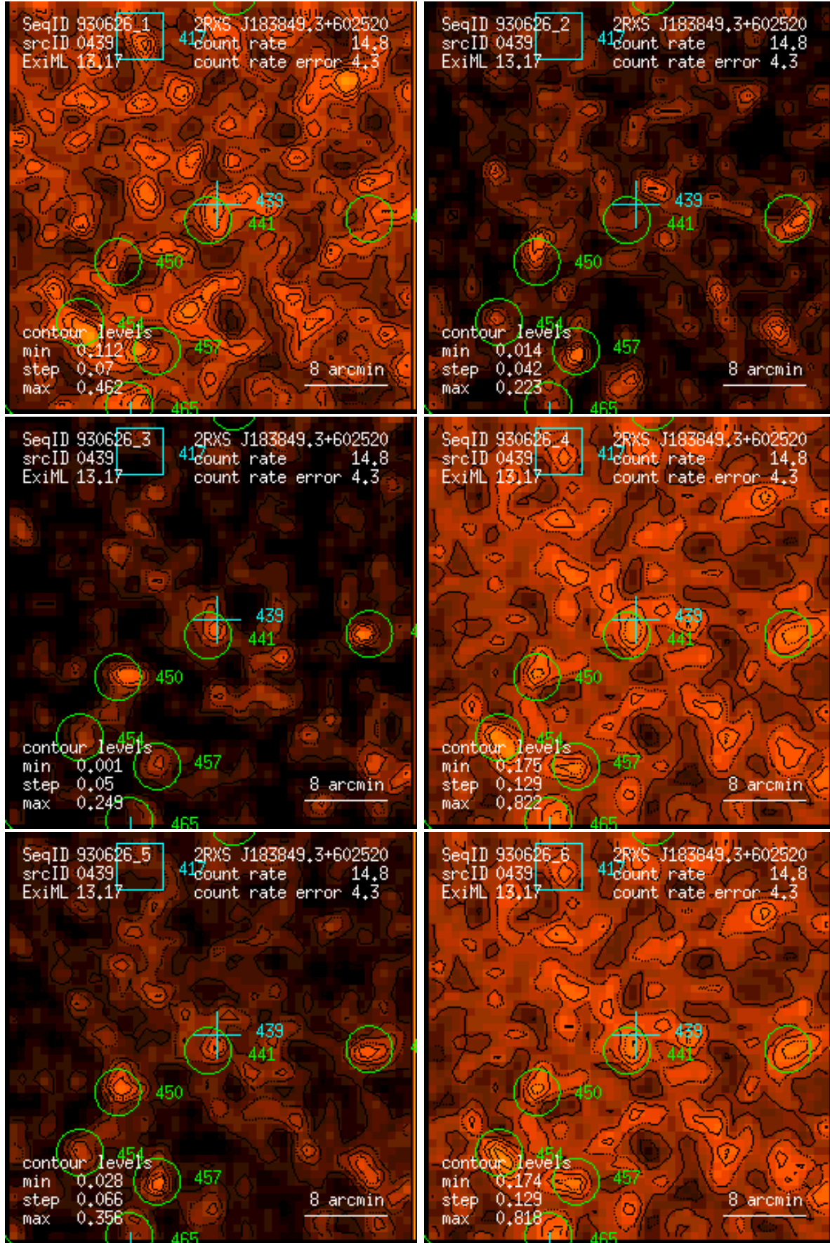
Figure 439: RASS 930626: detection 0439: band rate images, Gaussian filter: (1) PSPC channels 11 – 41, (2) 52 – 90, (3) 91 – 201, (4) 11 – 235, (5) 52 – 201, (6) 11 – 201. Broad band rates in counts/ks. Band rate contour levels in counts/ks/arcmin 2 .
