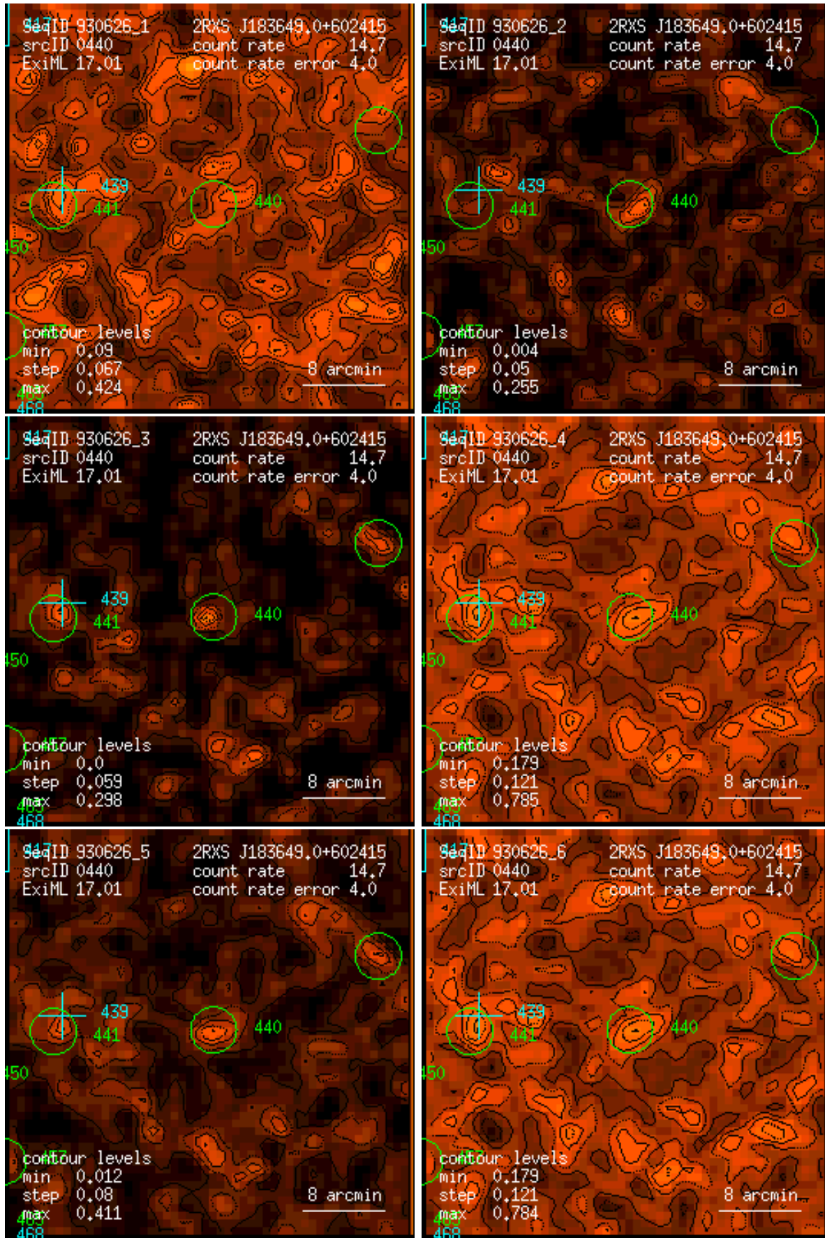
Figure 440: RASS 930626: detection 0440: band rate images, Gaussian filter: (1) PSPC channels 11 – 41, (2) 52 – 90, (3) 91 – 201, (4) 11 – 235, (5) 52 – 201, (6) 11 – 201. Broad band rates in counts/ks. Band rate contour levels in counts/ks/arcmin 2 .
