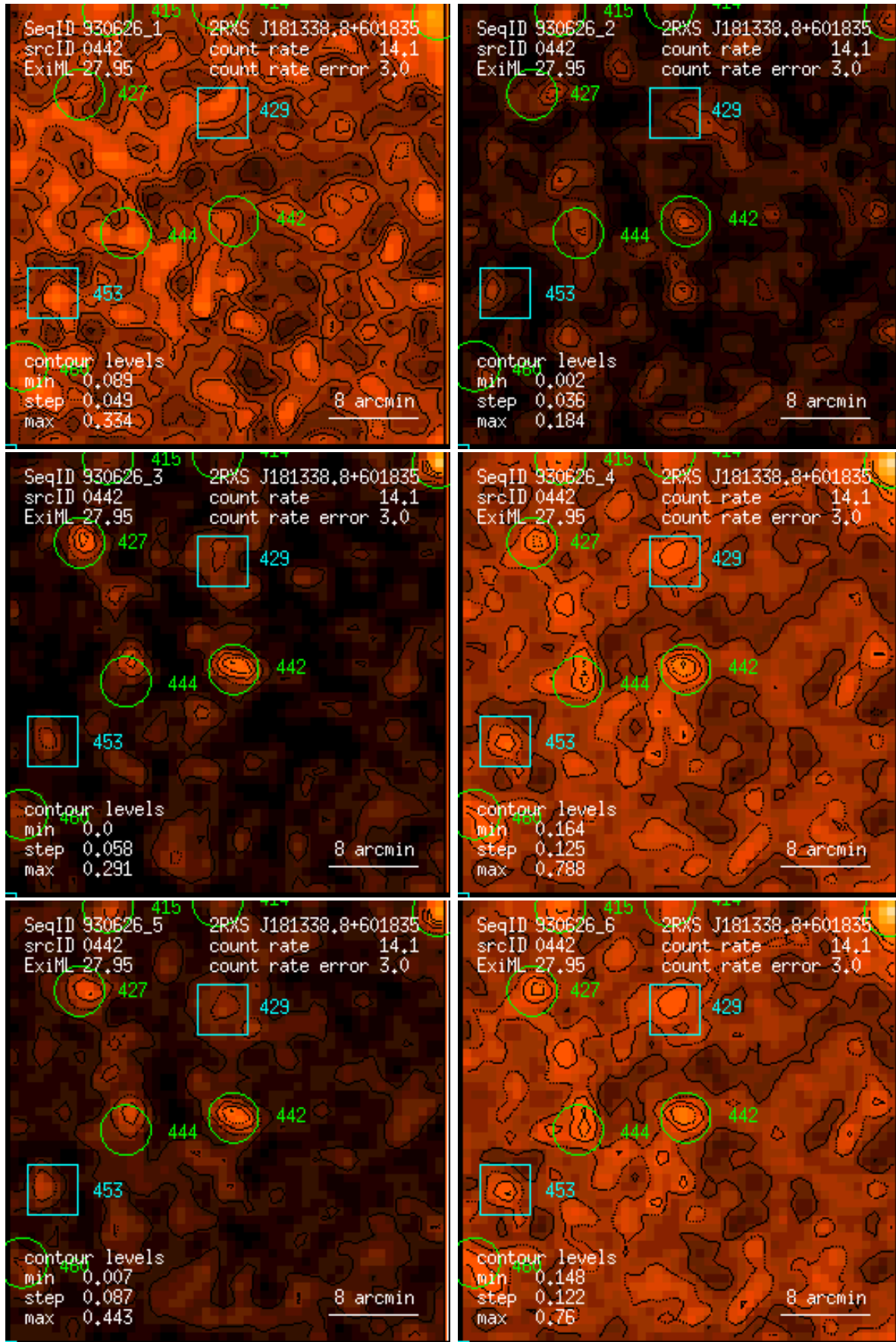
Figure 442: RASS 930626: detection 0442: band rate images, Gaussian filter: (1) PSPC channels 11 – 41, (2) 52 – 90, (3) 91 – 201, (4) 11 – 235, (5) 52 – 201, (6) 11 – 201. Broad band rates in counts/ks. Band rate contour levels in counts/ks/arcmin 2 .
