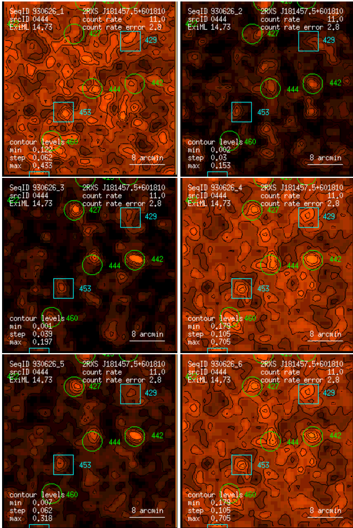
Figure 444: RASS 930626: detection 0444: band rate images, Gaussian filter: (1) PSPC channels 11 – 41, (2) 52 – 90, (3) 91 – 201, (4) 11 – 235, (5) 52 – 201, (6) 11 – 201. Broad band rates in counts/ks. Band rate contour levels in counts/ks/arcmin 2 .
