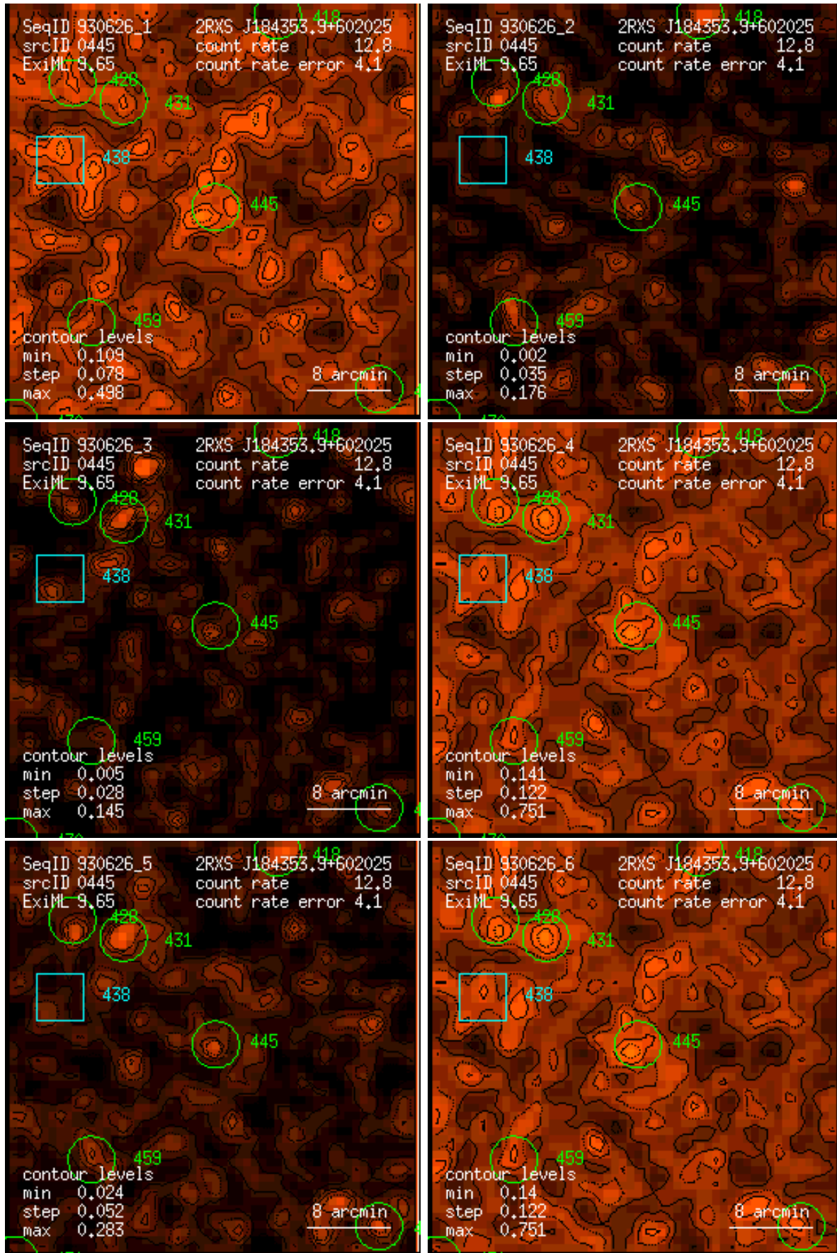
Figure 445: RASS 930626: detection 0445: band rate images, Gaussian filter: (1) PSPC channels 11 – 41, (2) 52 – 90, (3) 91 – 201, (4) 11 – 235, (5) 52 – 201, (6) 11 – 201. Broad band rates in counts/ks. Band rate contour levels in counts/ks/arcmin 2 .
