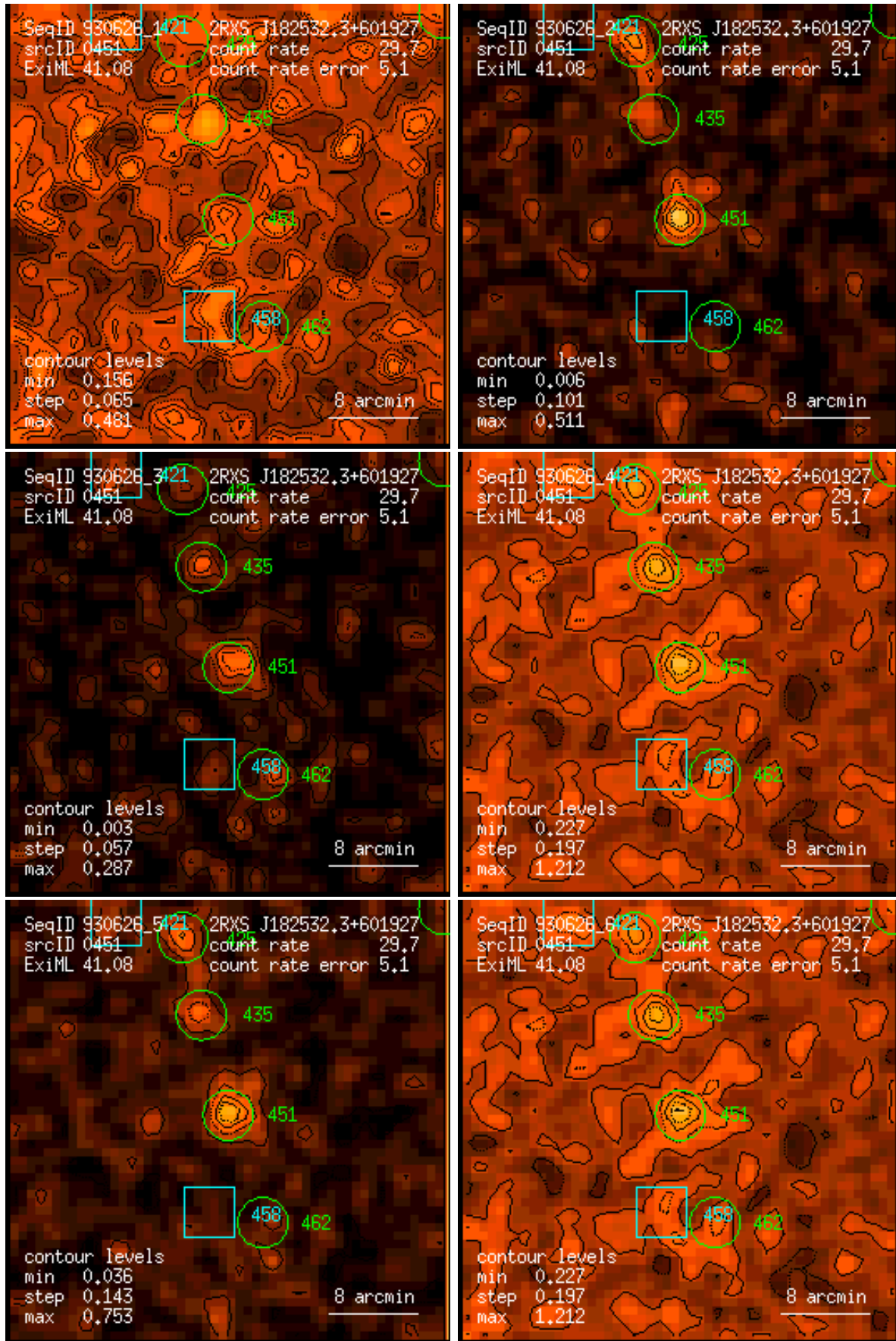
Figure 451: RASS 930626: detection 0451: band rate images, Gaussian filter: (1) PSPC channels 11 – 41, (2) 52 – 90, (3) 91 – 201, (4) 11 – 235, (5) 52 – 201, (6) 11 – 201. Broad band rates in counts/ks. Band rate contour levels in counts/ks/arcmin 2 .
