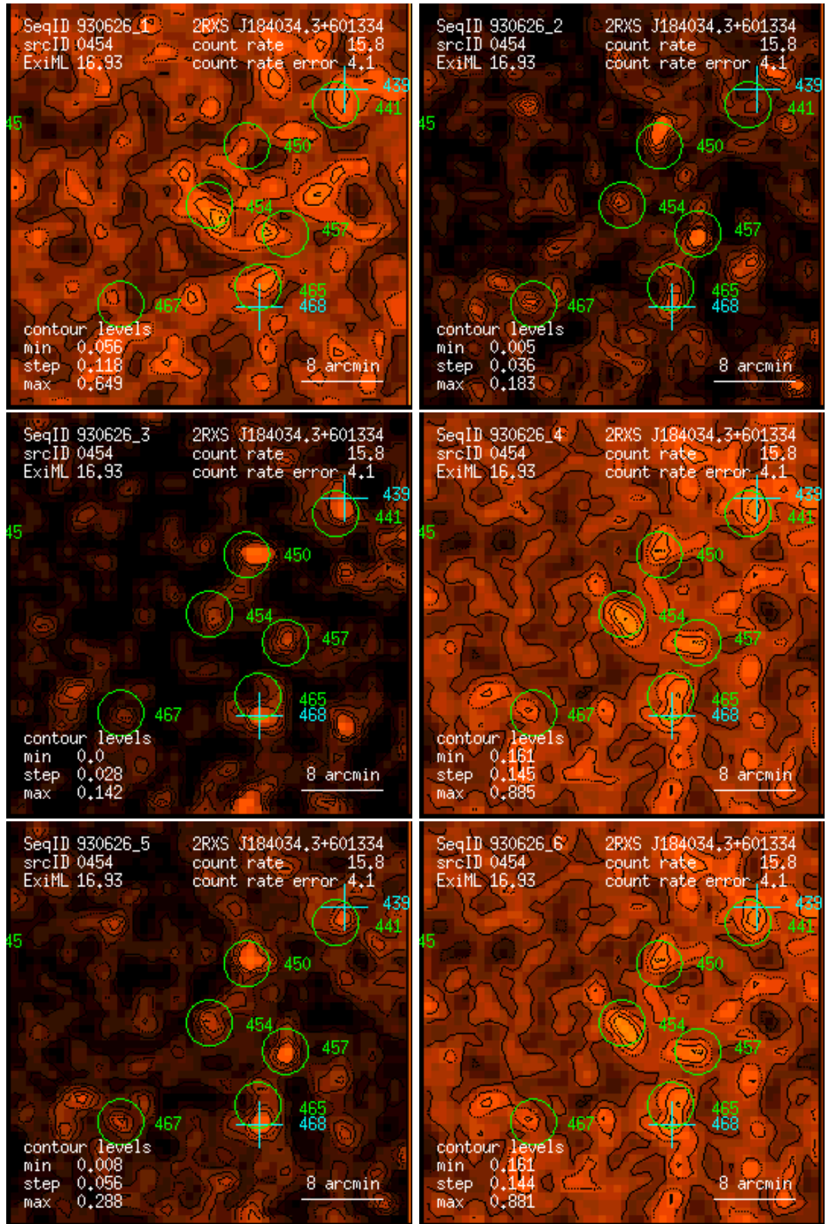
Figure 454: RASS 930626: detection 0454: band rate images, Gaussian filter: (1) PSPC channels 11 – 41, (2) 52 – 90, (3) 91 – 201, (4) 11 – 235, (5) 52 – 201, (6) 11 – 201. Broad band rates in counts/ks. Band rate contour levels in counts/ks/arcmin 2 .
