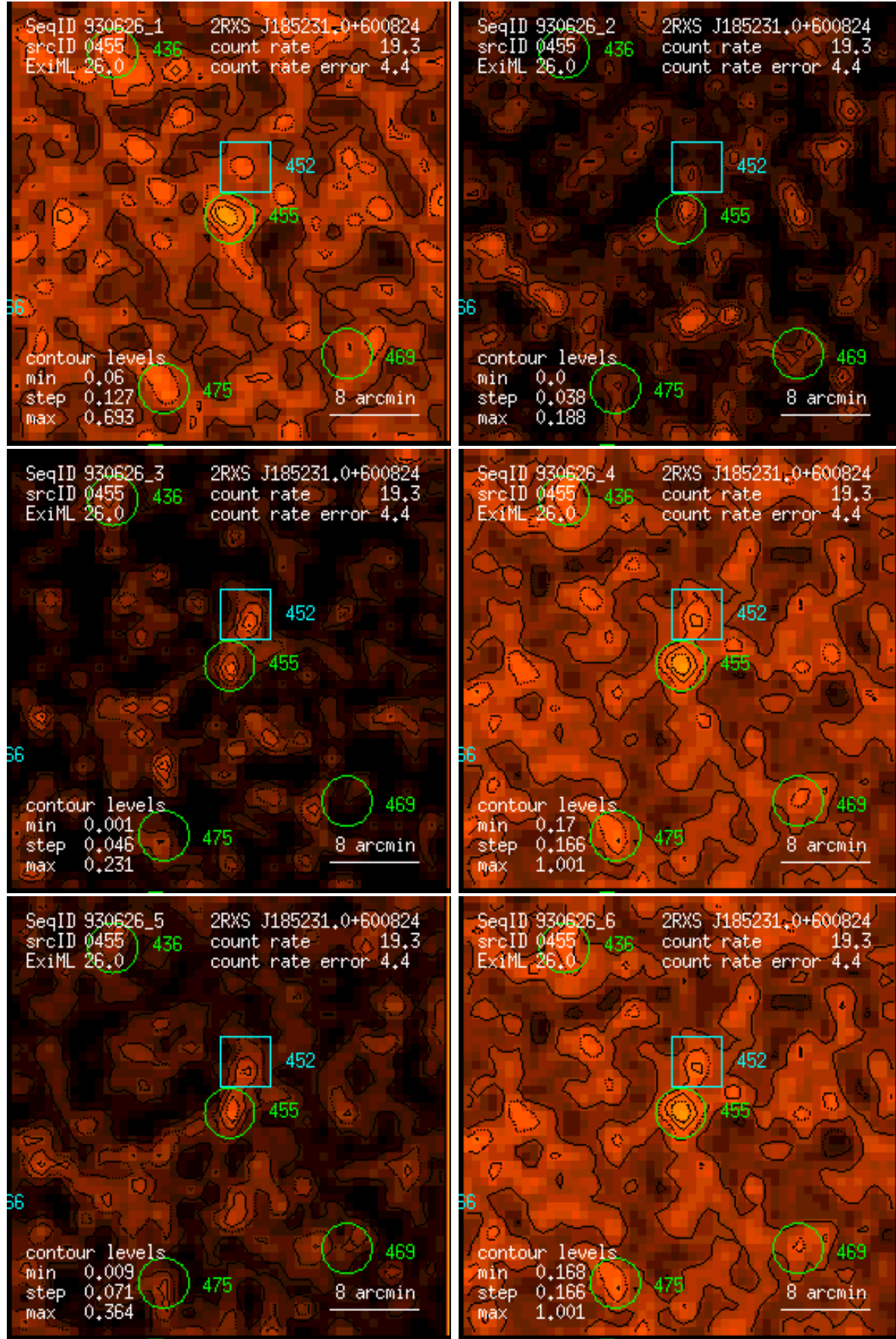
Figure 455: RASS 930626: detection 0455: band rate images, Gaussian filter: (1) PSPC channels 11 – 41, (2) 52 – 90, (3) 91 – 201, (4) 11 – 235, (5) 52 – 201, (6) 11 – 201. Broad band rates in counts/ks. Band rate contour levels in counts/ks/arcmin 2 .
