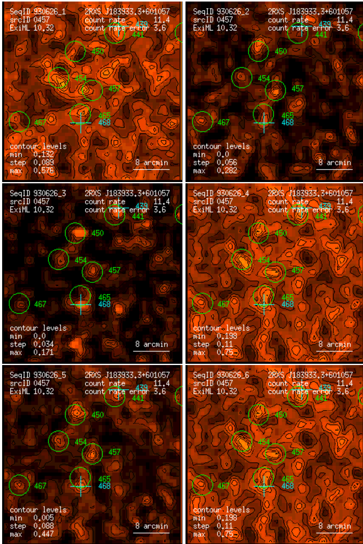
Figure 457: RASS 930626: detection 0457: band rate images, Gaussian filter: (1) PSPC channels 11 – 41, (2) 52 – 90, (3) 91 – 201, (4) 11 – 235, (5) 52 – 201, (6) 11 – 201. Broad band rates in counts/ks. Band rate contour levels in counts/ks/arcmin 2 .
