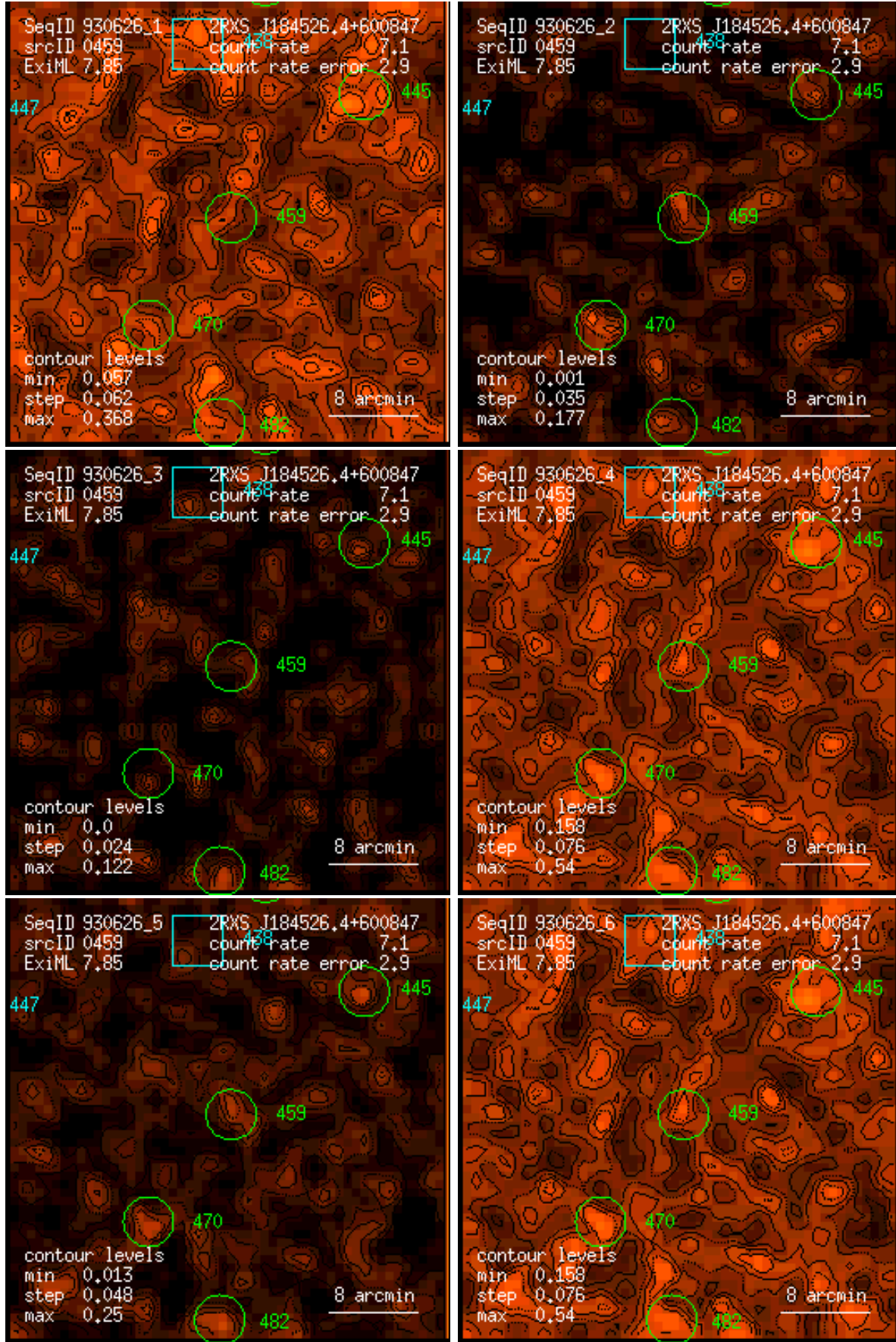
Figure 459: RASS 930626: detection 0459: band rate images, Gaussian filter: (1) PSPC channels 11 – 41, (2) 52 – 90, (3) 91 – 201, (4) 11 – 235, (5) 52 – 201, (6) 11 – 201. Broad band rates in counts/ks. Band rate contour levels in counts/ks/arcmin 2 .
