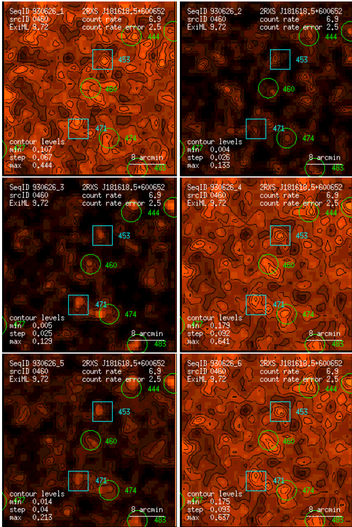
Figure 460: RASS 930626: detection 0460: band rate images, Gaussian filter: (1) PSPC channels 11 – 41, (2) 52 – 90, (3) 91 – 201, (4) 11 – 235, (5) 52 – 201, (6) 11 – 201. Broad band rates in counts/ks. Band rate contour levels in counts/ks/arcmin 2 .
