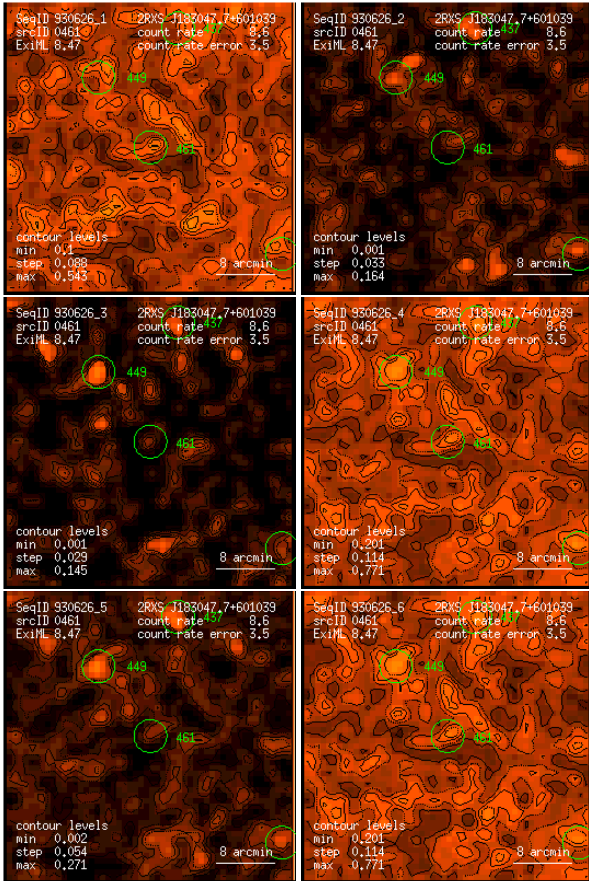
Figure 461: RASS 930626: detection 0461: band rate images, Gaussian filter: (1) PSPC channels 11 – 41, (2) 52 – 90, (3) 91 – 201, (4) 11 – 235, (5) 52 – 201, (6) 11 – 201. Broad band rates in counts/ks. Band rate contour levels in counts/ks/arcmin 2 .
