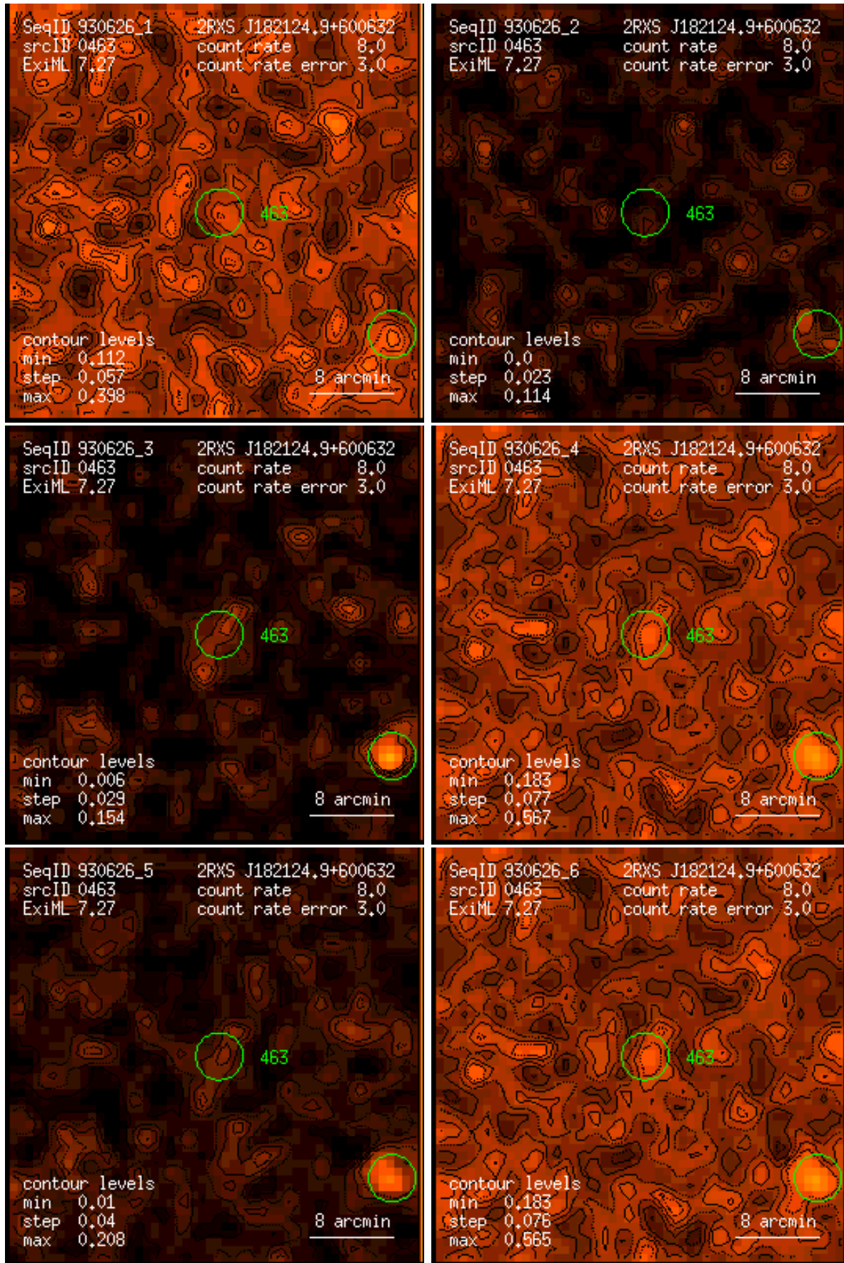
Figure 463: RASS 930626: detection 0463: band rate images, Gaussian filter: (1) PSPC channels 11 – 41, (2) 52 – 90, (3) 91 – 201, (4) 11 – 235, (5) 52 – 201, (6) 11 – 201. Broad band rates in counts/ks. Band rate contour levels in counts/ks/arcmin 2 .
