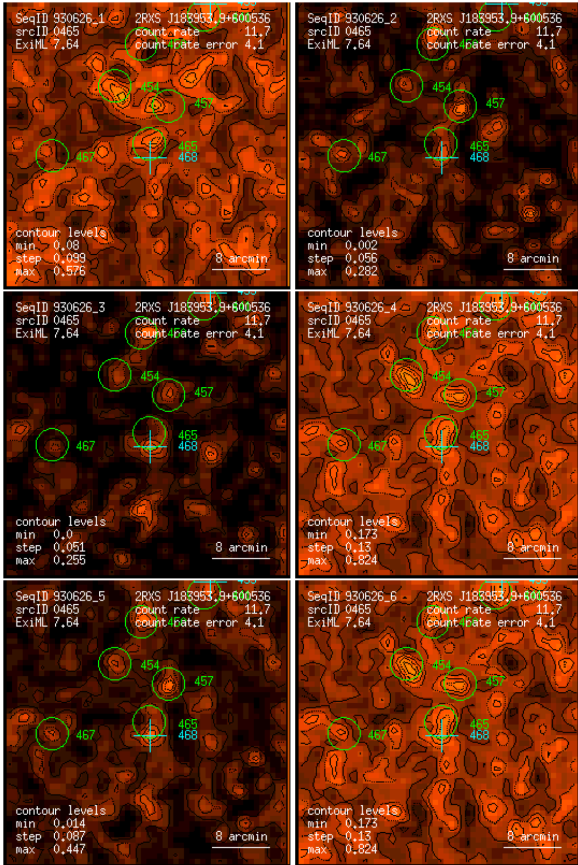
Figure 465: RASS 930626: detection 0465: band rate images, Gaussian filter: (1) PSPC channels 11 – 41, (2) 52 – 90, (3) 91 – 201, (4) 11 – 235, (5) 52 – 201, (6) 11 – 201. Broad band rates in counts/ks. Band rate contour levels in counts/ks/arcmin 2 .
