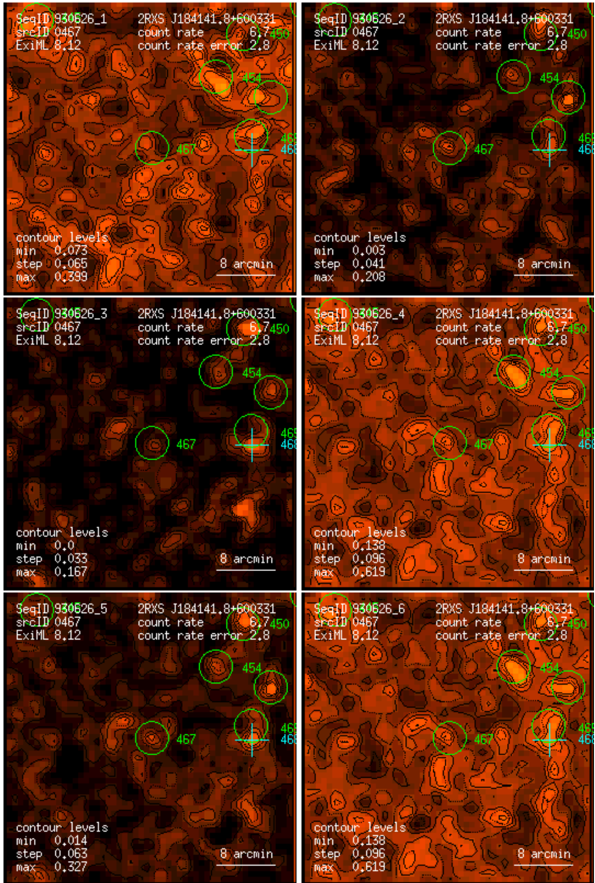
Figure 467: RASS 930626: detection 0467: band rate images, Gaussian filter: (1) PSPC channels 11 – 41, (2) 52 – 90, (3) 91 – 201, (4) 11 – 235, (5) 52 – 201, (6) 11 – 201. Broad band rates in counts/ks. Band rate contour levels in counts/ks/arcmin 2 .
